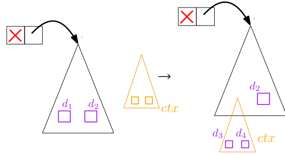
Figure 4. refine filling a destiny with a structure that has holes. It allocates destinies to the holes of the structure, and returns them.
