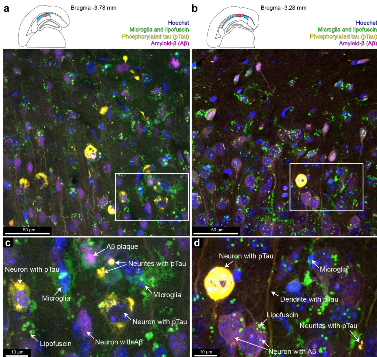
Figure 2. Four-color detergent-free immunofluorescence enabled by nanobody probes.
