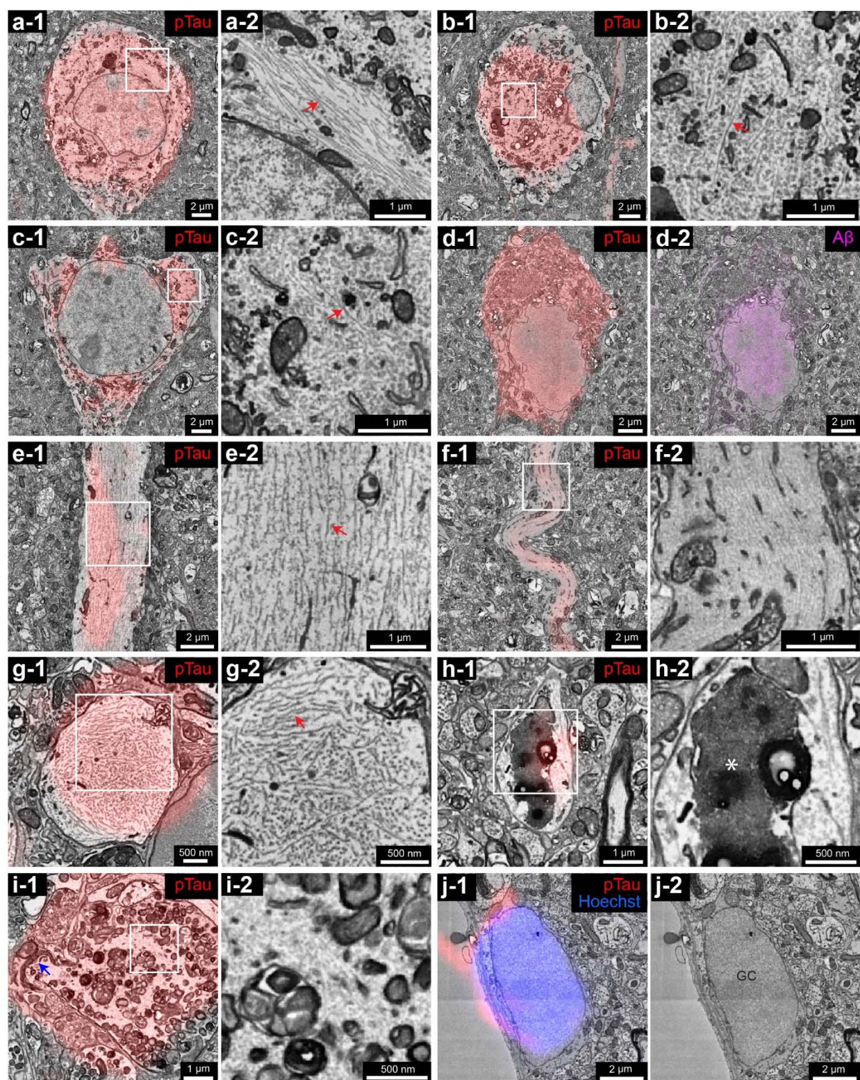
Figure 5. Ultrastructural abnormalities related to the anti-pTau nanobody labeling.
