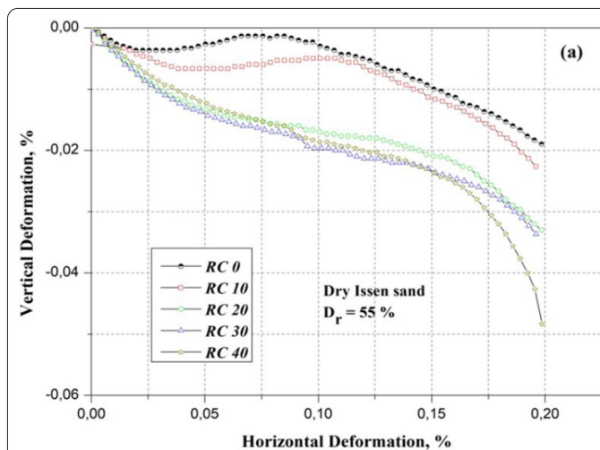
Figure 6: Correlation between horizontal and vertical deformation for varied rubber contents under 200 kPa normal stress: (a) Dry sand and (b) saturated sand.
