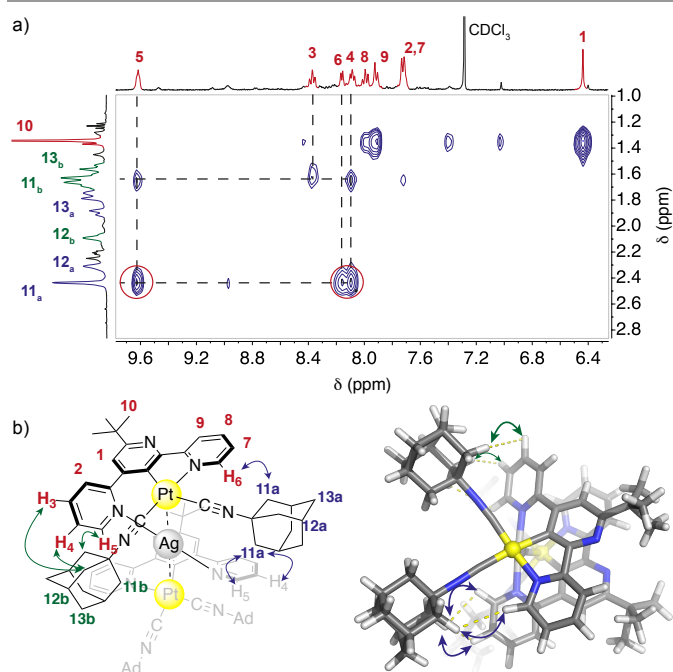
Figure 4. a) 1 H NMR NOESY Spectra (600 MHz, CDCl 3 , 300K) of dimer 3 showing correlation between adamantyl protons H 1,1a and pyridine protons H 6 and H 4,5 of both Pt(II) moieties. b) representation of selected correlation in the crystallographic structure.
