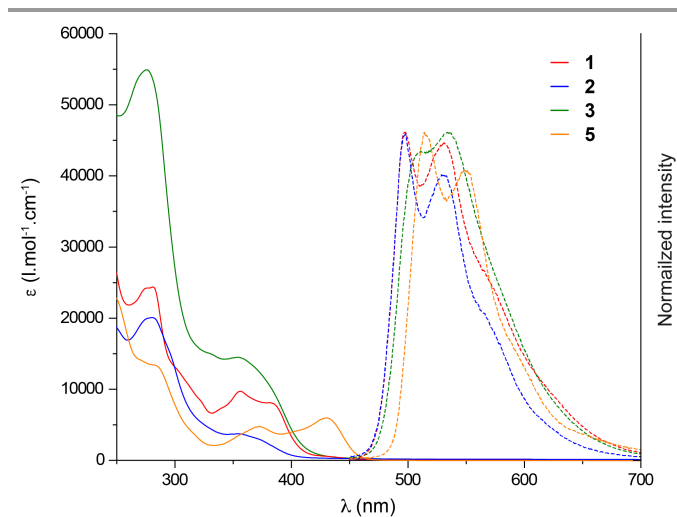
Figure 5. Absorption and normalized emission spectra (dashed) of complexes 1 , 2 and 3 , (5 × 10 -5 mol.l -1 in CHCl 3 , 298 K, λ exc = 400 nm).
