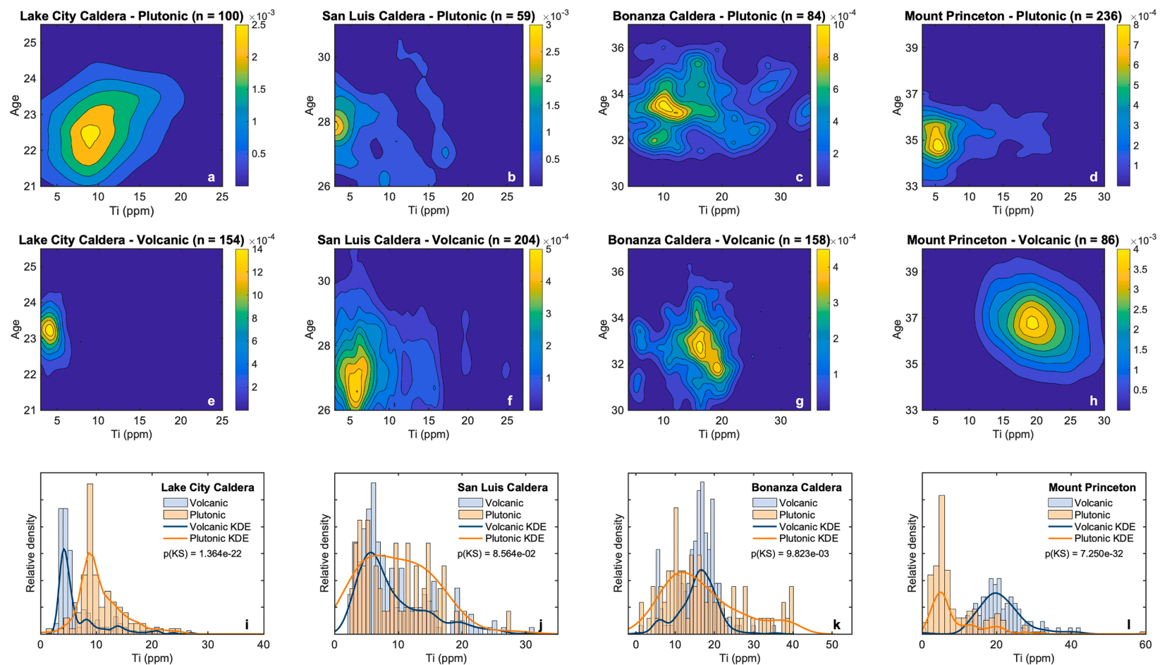
Fig. 2. Summary of LA-ICP-MS 206 Pb/ 238 U age and Ti content from zircons in plutonic and volcanic units from the Southern Rocky Mountain volcanic field (Lake City Caldera, San Luis Caldera, Bonanza Caldera, Mt Princeton). (A-D) corresponds to combined age and Ti content density plots. (I-L) shows combined kernel density estimations (KDEs) and histograms. Result of Kolmogorov-Smirnov (KS) statistical analyses is shown as p(KS), with the low value indicating that the two populations are unlikely to be derived from the same underlying distribution.
