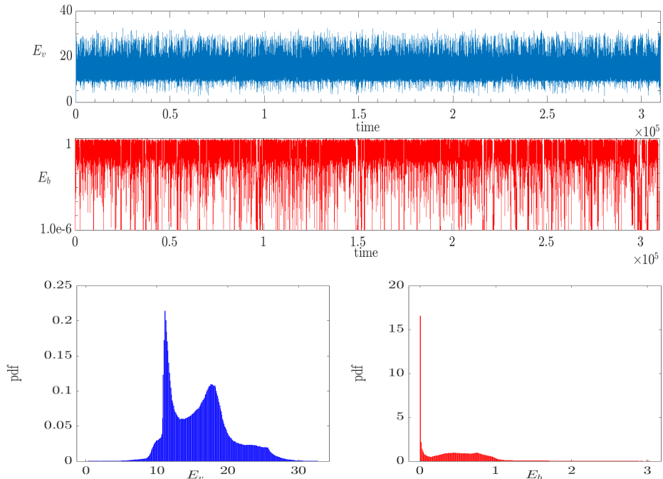
FIGURE 1. Run ABC2: temporal evolutions of the kinetic energy (blue, top) and magnetic energy (red, middle). Bottom: Probability density functions of the kinetic energy (left) and magnetic energy (right). Note the different units on the axes, and the lin-log scale for the magnetic energy.
