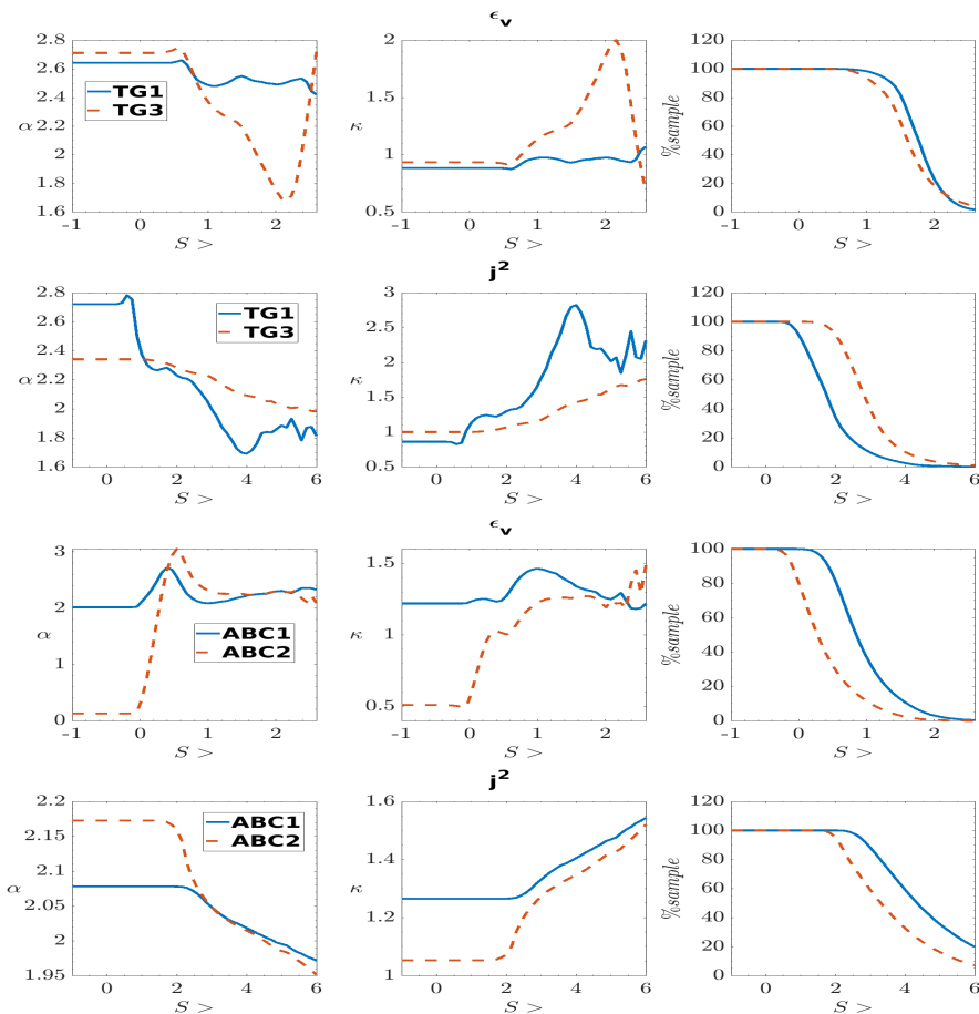
FIGURE 6. Given a fit |K(S)| \sim \kappa|S|^\alpha , variations with filter level in S of the parameters \alpha (left), \kappa (middle) and the percentage of available data points per filter level in S (right), for \epsilon_v (first and third rows) and j^2 (second and fourth rows), for the two TG runs (first two rows) and the two ABC runs (last two rows), with line and colors indicated in the inserts.
