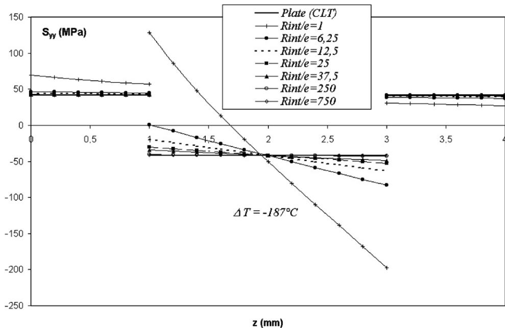
Fig. 18. Thermal stress S_{yy} induced in a [0/90]_S plates and cylinders by a uniform temperature differential \Delta T = -187^\circ\text{C} .
