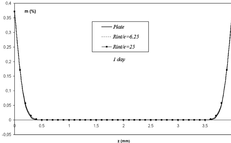
Fig. 10. Plate and cylinder hygroscopic fields after one day conditioning at T = 23 °C and HR% = 50%.
