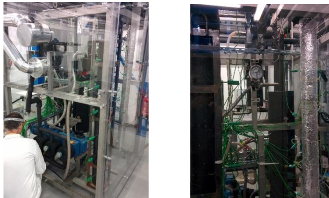
Fig. 7. Photographs of CO 2 loop and two vertical test sections
