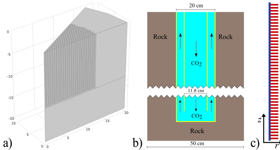
Fig 3. a) Drawing of a 30° sector of the ground heat storage, b) sketch of a single coaxial exchanger, c) 1D/2D computational model (deformed in the radial direction) - fluid domain (blue) and rock domains (red)
