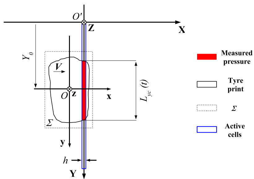
Fig. 5. Position of the active line of cells for the "transverse tests".
