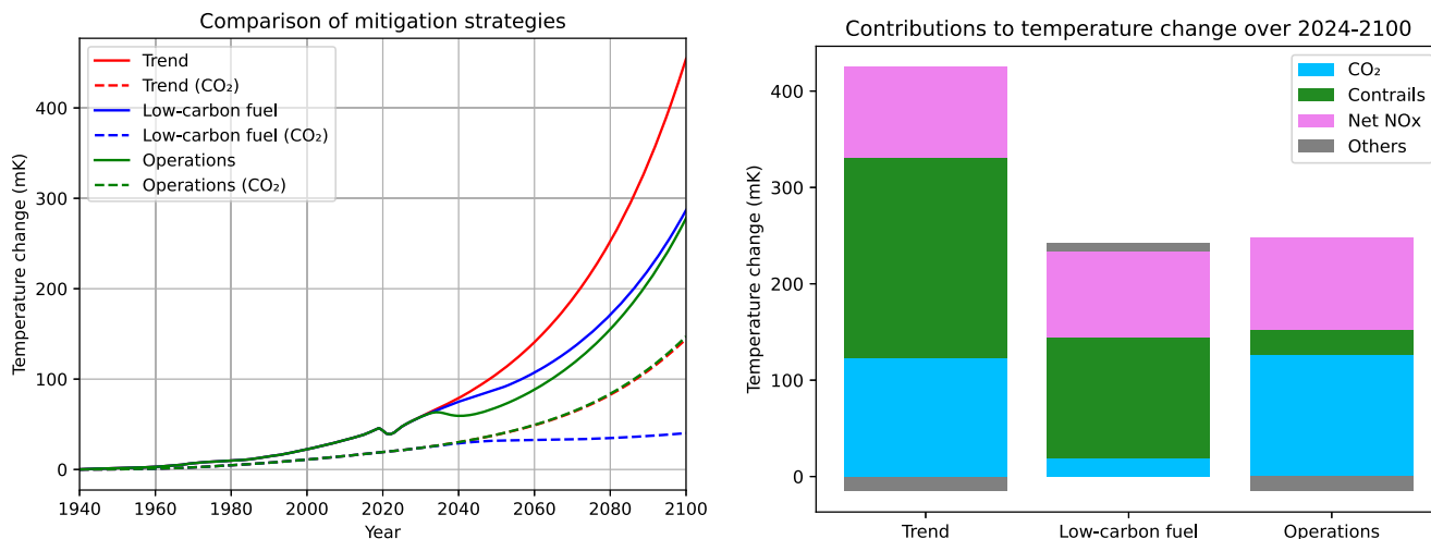
Fig. 5 | Aviation’s contribution to surface temperature change from 1940 until 2100 across three future scenarios with 3% aviation growth. 1/ Trend (exclusive use of kerosene), 2/ Low-carbon fuel (adoption of low-carbon fuels by 2050),
