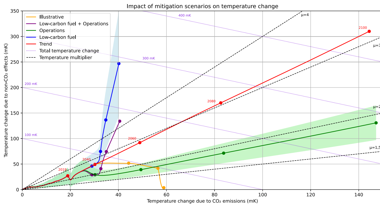
Fig. 7 | Comparison of the surface temperature change of mitigation scenarios. The graph allows their direct comparison, showing the contribution of CO 2 emissions and non-CO 2 effects to temperature change on the x- and y-axis. Total
