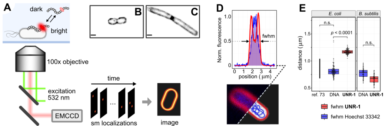
Figure 4. A) Single-molecule localization microscopy with UNR-1 . B–C) Super-resolution fluorescence microscopy images of UNR-1 -labeled E. coli ( B ) and B. subtilis ( C ); scale bars, 1 μm. D) Normalized fluorescence intensity profiles obtained from two-color confocal fluorescence images of bacteria co-labeled with UNR-1 (red) and Hoechst 33342 (blue); fwhm = full width at half-maximum. E) Comparison of the fwhm values of the red and blue fluorescence intensity profiles for E. coli and B. subtilis ( n > 50 cells, one-tailed Wilcoxon–Mann–Whitney test, n.s. = non-significant); reference diameter of E. coli cells was taken from ref. 73
