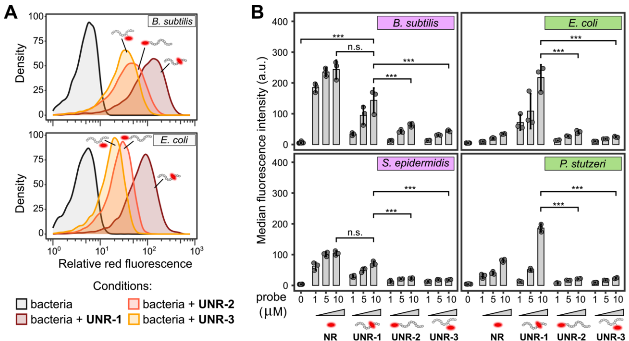
Figure 2. Flow cytometry analysis of bacteria stained with NR and the NR -labeled peptidic probes. A) Flow cytometry profiles of the representative Gram-positive and Gram-negative bacteria incubated with the peptidic probes UNR-1 , UNR-2 and UNR-3 ; the labeling was performed under no-wash conditions by adding the probe (5 \mu\text{M} ) to the bacteria in the early logarithmic phase shortly before measurements; excitation wavelength was 488 nm; fluorescence was detected using a 680/30 emission filter. B) Mean of median fluorescence intensities of the bacteria stained with 1, 5, and 10 \mu\text{M} of NR and the NR -based
