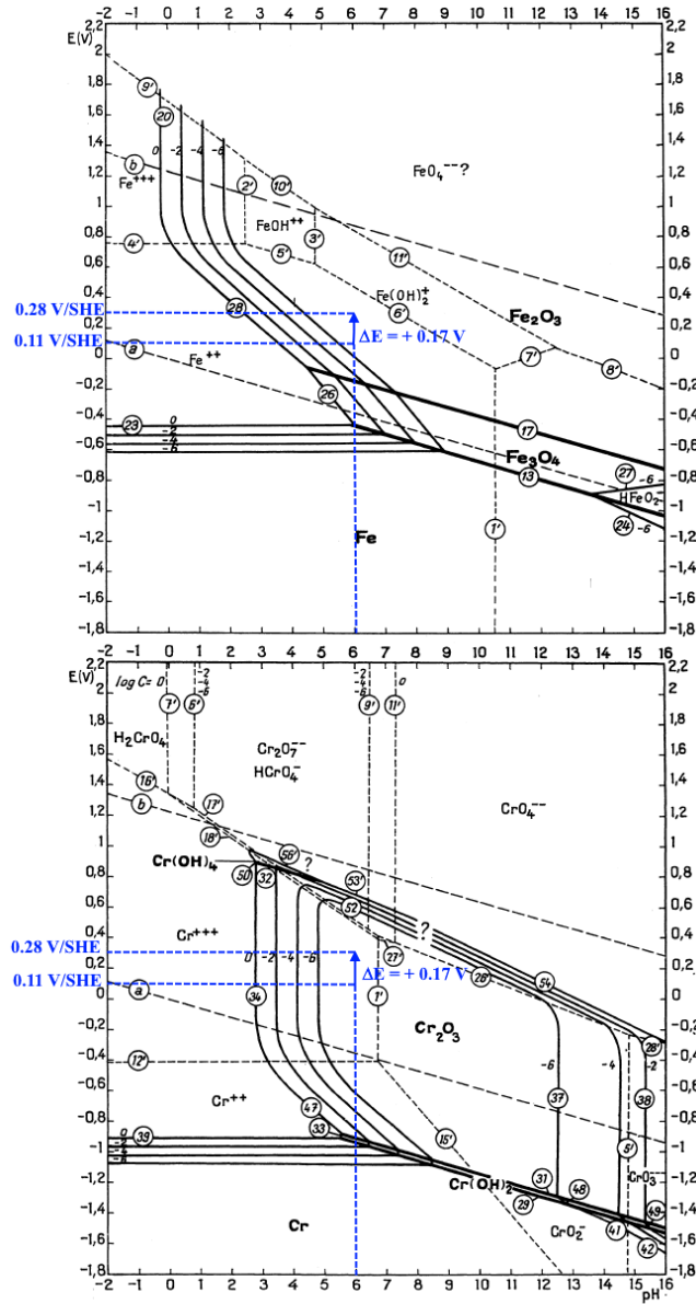
Figure 3: Pourbaix diagrams [76] at 25 °C a) of iron and b) of chromium. The blue arrow represents on both diagrams the potential difference \Delta E = +0.17 \text{ V} . (SHE: Standard Hydrogen Electrode). Reprinted with permission from AMPP from "Atlas of Electrochemical Equilibria in Aqueous Solutions", M. Pourbaix, 1974.
