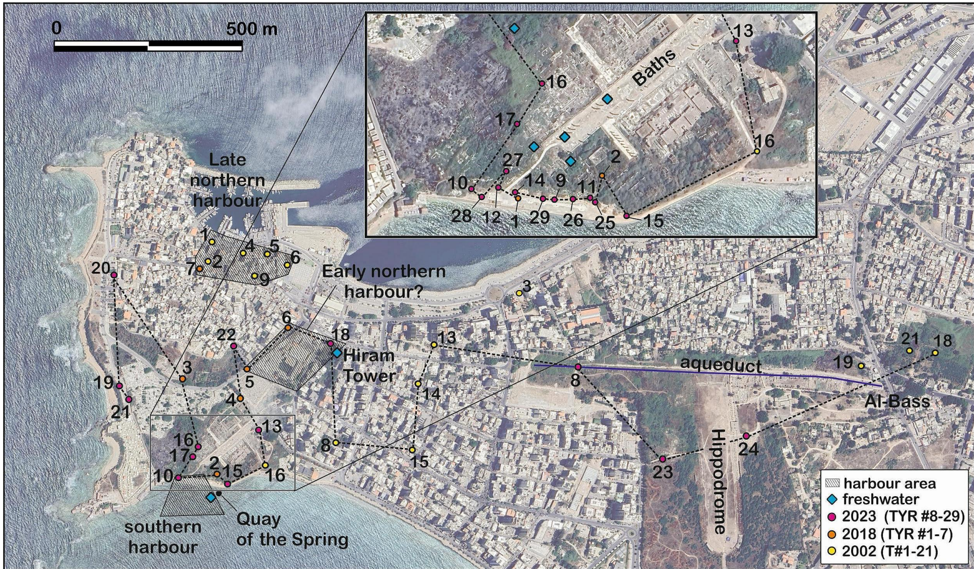
Fig. 2. Location of the 2023 coring sites and earlier coring sites along the peninsula of Tyre. Dashed line: transect followed for stratigraphic correlations on fig. 4. Background: satellite image © 2024 Airbus, accessed via Google Earth Pro 7.3.6.9750, version of January 12th 2024.
