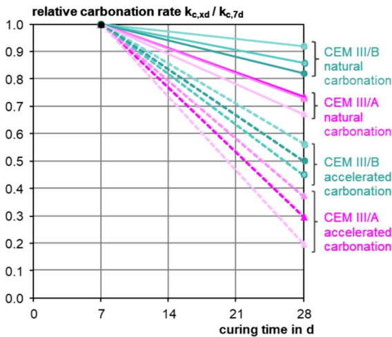
Fig. 18 Relative carbonation coefficient k_{c,xd \text{ curing}} / k_{c,7d \text{ curing}} versus number of curing days for mixes with same composition exposed to natural (solid lines) and accelerated (dashed lines) carbonation
