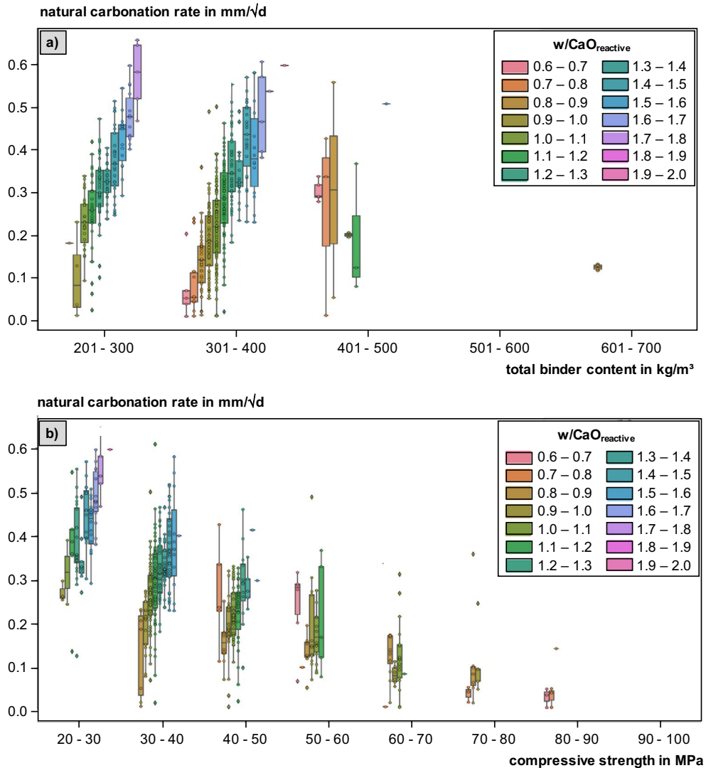
Fig. 11 Natural carbonation rate versus range of (a) total binder content and (b) compressive strength range (28 d, 150 mm cubes) for clusters based on w/CaO_{reactive}
