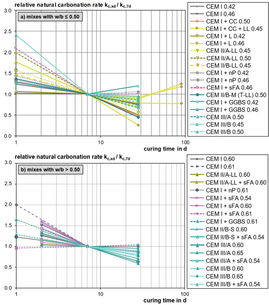
Fig. 17 Relative carbonation coefficient k_{c,xd}/k_{c,7d} versus curing duration for mixes with different composition exposed to natural carbonation Note: Same labelling for different results can be derived from the fact that the labelling only mentions binder type and w/b value but other parameters were also varied (for example different studies could have used similar compositions or further parameters were varied such as the SCM content)
