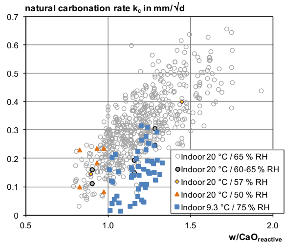
Fig. 20 Carbonation rate vs. w/\text{CaO}_{\text{reactive}} for indoor natural carbonation at different temperatures and relative humidities (RH)
