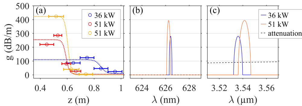
Figure 4. (a) Experimental gain measurements for the anti-Stokes wave centred at 0.625\ \mu\text{m} as a function of propagation distance z , obtained for peak powers in the fundamental mode equal to 51 kW (red and yellow) and 36 kW (blue) (with fitting curves in dashed lines as guides to the eye). Horizontal solid segments also indicate the cutback fiber lengths. (b and c) Theoretical gain calculations for the anti-Stokes (b) and Stokes (c) waves for 36 kW (blue) and 51 kW (orange) peak power. Black dashed line indicates the value of fiber attenuation in this spectral region.
