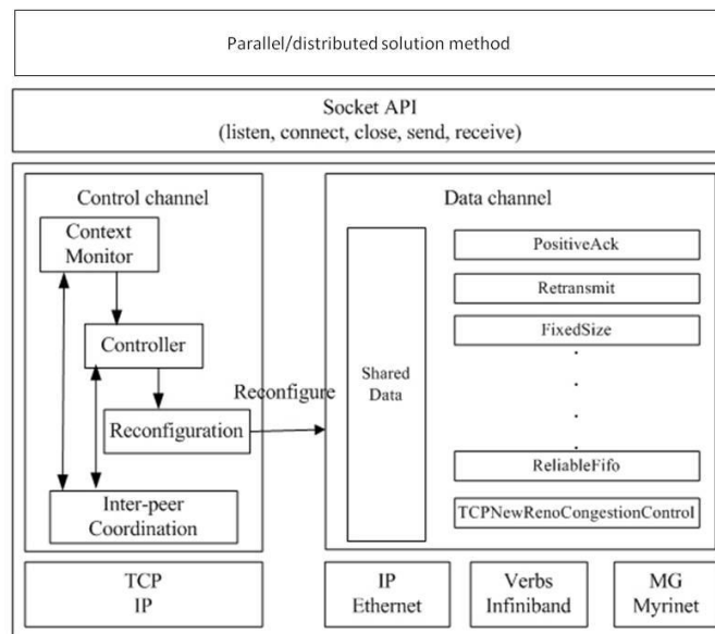
Figure 2. P2PSAP protocol architecture.
