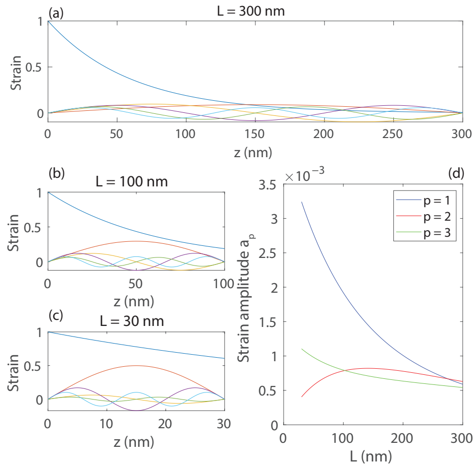
Figure 2. Illustration of the first few acoustic eigenmode profiles (normalized) for (a) L = 300 nm, (b) L = 100 nm and (c) L = 30 nm. In each graph, the blue line indicates the overall strain profile, while the other lines indicate the eigenmode components with their respective amplitudes. (d) Strain amplitudes a_p(L) , for the first three modes p = 1, 2, 3 .
