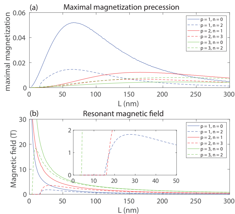
Figure 4. (a) Peak magnetization amplitude dependence on film thickness for different phonon–magnon pairs ( p, n ). (b) Magnetic field necessary for resonant interaction versus film thickness for different phonon–magnon pairs ( p, n ). The inset shows the same graph restricted to experimentally feasible magnetic fields in the range of 0 T–2 T and to film thicknesses between 0 and 50 nm. A prominent feature is the sudden fall to zero of the magnetic field necessary to achieve a magnon resonance for film thicknesses of 16 nm ( p = 1, n = 0 and p = 2, n = 1 ) and 3 nm, respectively ( p = 3, n = 0 ).
