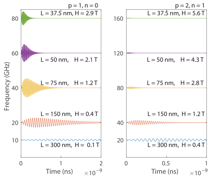
Figure 3. Magneto-acoustic resonances of different acoustic p and magnetic n orders behave differently as the thickness of a freestanding nickel layer decreases. Acoustically driven magnetization precession of p = 1 -driven n = 0 (FMR) and p = 2 -driven n = 1 (magnon) precession for different values of film thickness L ( L = 300 nm, L = 150 nm, L = 75 nm, L = 50 nm and L = 37.5 nm). The required magnetic field values are indicated next to each curve.
