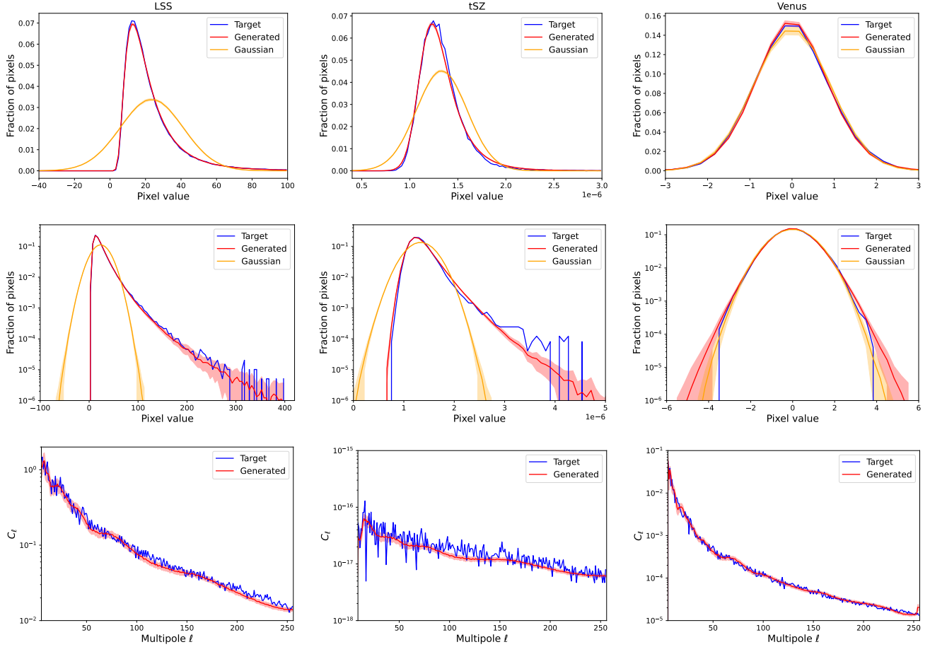
Fig. 5. Statistical validation. The PDF and angular power spectra for the LSS, tSZ, and Venus fields (left to right). The first row shows the PDF with a linear y -axis scaling, while the second row shows the same PDF with a logarithmic y -axis. The third row shows the angular power spectra. The target is shown in blue, the generated fields in red, and the Gaussian realisations in yellow. We plotted the mean (solid line) and the standard deviation (shadow envelope) over 50 realisations.
