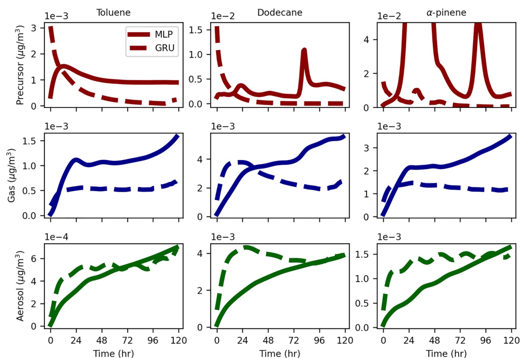
Figure 7. Mean ensemble standard deviation across all validation experiments as a function of simulation hour.
