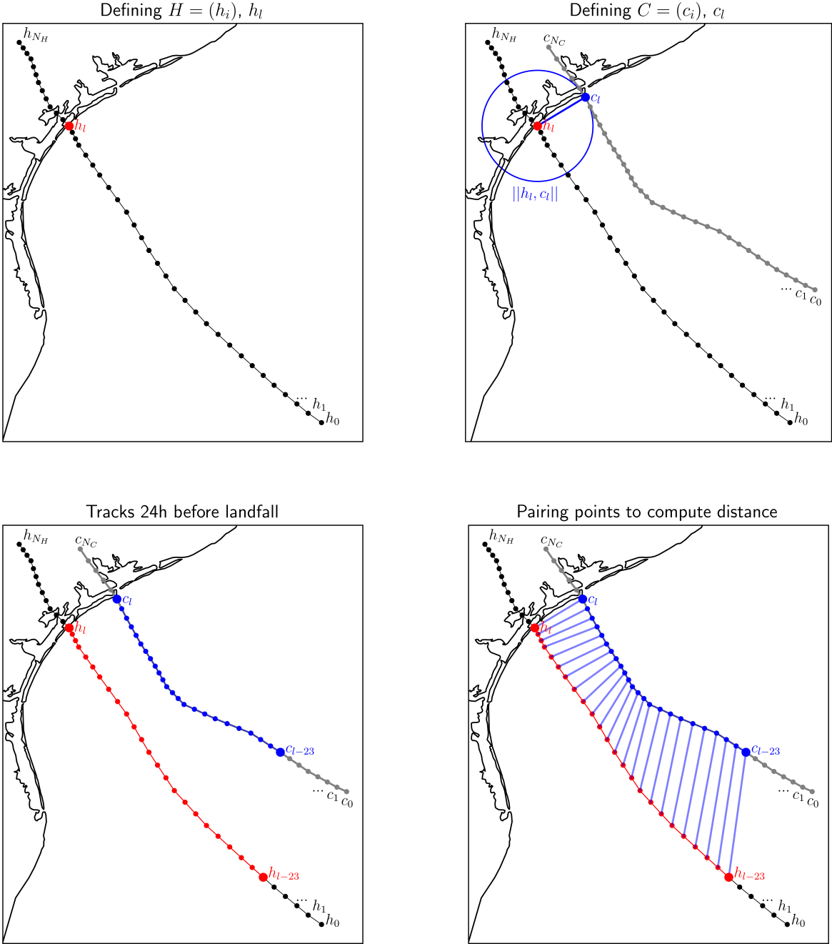
Figure A1. Illustration of the distance computation described in 3.2.2.
