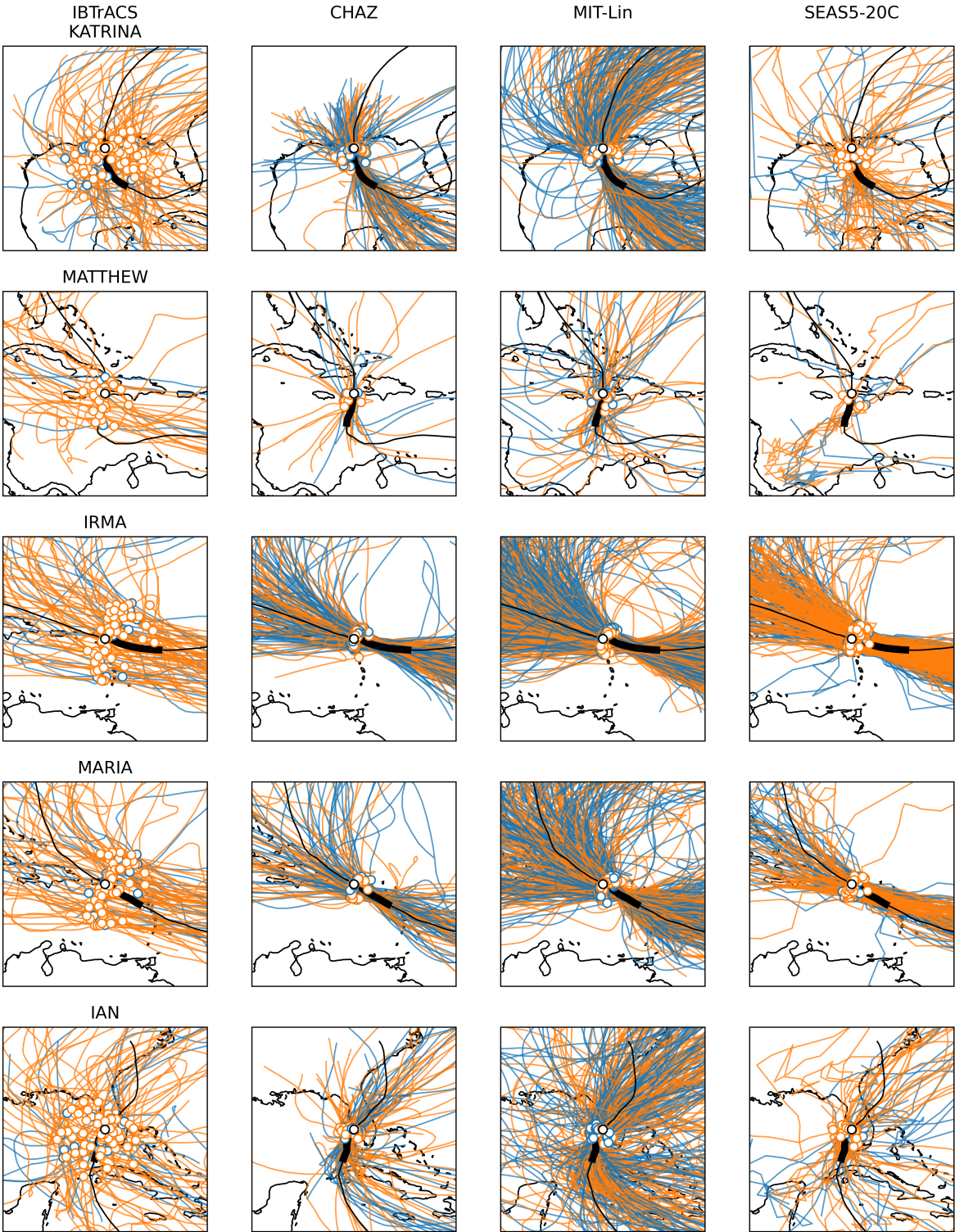
Figure A2. Same as figure 3 but for all 9 cases (continued in fig A3).
