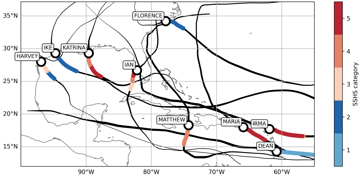
Figure 1. Hurricane cases in this study. Full tracks are shown in black with width proportional to intensity. Tracks 24h before landfall are colored by Saffir-Simpson Hurricane Scale (SSH) category. Dark circles show the landfall points considered in this study.
