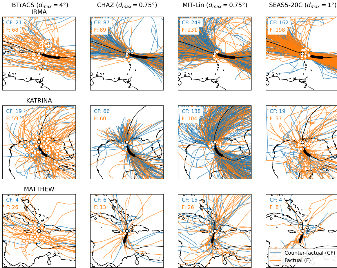
Figure 3. Analogues for hurricanes Irma (top), Katrina (middle) and Matthew (bottom), in each catalogue (columns). Counter-factual analogues are in blue and factual ones in orange. The black track is the observed hurricane track. The numbers on the top-left of each panel are the number of analogues for each period. Tracks for all analogues are shown in figures A2 & A3.
