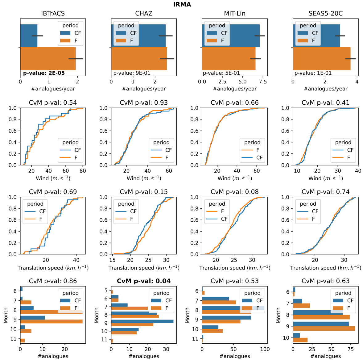
Figure 4. Characteristics of Irma’s analogues in each catalogue (columns). The first line shows the number of analogues per year for each period, with the error bar showing the standard error. The p-value is shown for a T-test for the mean, in bold when statistically significant at the 5% level. The second line shows the empirical cumulative distribution functions of maximum wind speed at the surface (for SEAS5-20C at 850hPa). The third line shows the empirical cumulative distribution functions of the translation speed during the 24 hours before landfall. The fourth line shows the month of the formation of the analogues in both periods. For lines 2–4, the results of a Cramer von Mises (CvM) test are shown, which determines whether the samples in each period are drawn from different distributions, in bold when the p-value is <5%. In the fourth line, the test was performed for the day-of-year.
