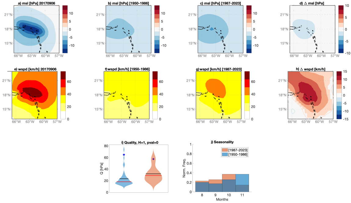
Figure 2. ERA5 Analogues Analysis for 6 September 2017 and the region defined by [66.9W 56.9W 12.7E 22.7E] and the hurricane season ASON.
