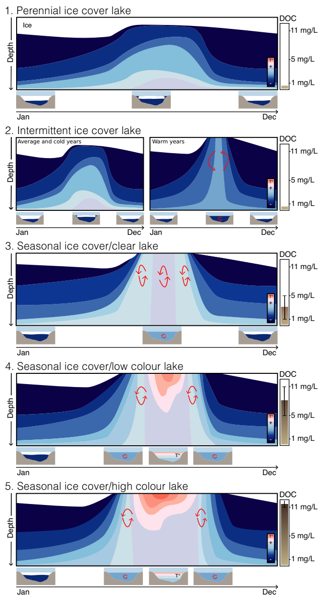
Fig. 5 | Lake contrasting states found along the transect. Along the latitudinal transect, freshwater lakes (the typical lake defined for the study region has an average area of 24 ha and a mean depth of 4.0 m – see Supplementary Note 1) range from perennially frozen clear lakes to lakes with seasonal ice cover and high dissolved organic matter content. Lake contrasting states are defined by the duration of ice cover, stratification of the water column and mixing regime, oxygen and light availability, as well as the dissolved organic matter content (given as dissolved organic carbon, or DOC).
