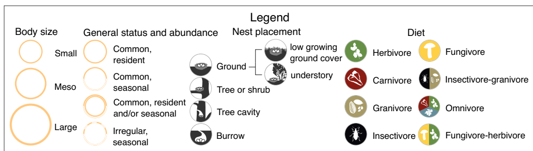
Fig. 8 | Endothermic vertebrates contrasting states found along the transect. Along the latitudinal transect, endothermic terrestrial vertebrate communities range from an assemblage of few functional groups in the High-Arctic to a highly functionally diverse boreal vertebrate community. Contrasting states are defined by the occurrence and relative abundance of mammalian and avian functional groups present and active in the landscape (100 km x 100 km, a scale that encompasses
