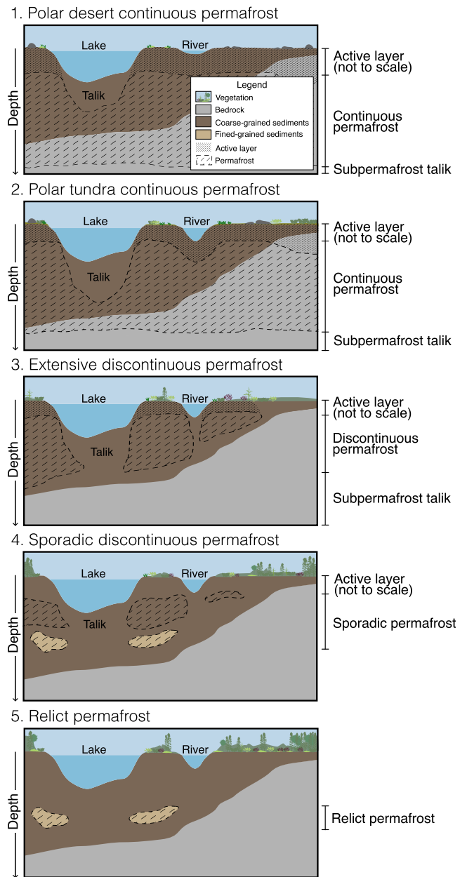
Fig. 3 | Permafrost contrasting states found along the transect. Permafrost is defined as rock or soil that remains below 0°C for at least two consecutive years. Along the latitudinal transect, it ranges from extensive continuous thick permafrost to relict permafrost located in isolated underground patches. Permafrost contrasting states are primarily based on the extent of frozen ground across the landscape (30 km X 30 km). States are also described using the characteristics (temperature, permafrost thickness, water and ice contents) of their different layers (active layer, perennially frozen ground and taliks – see Supplementary Note 1 for definitions).
