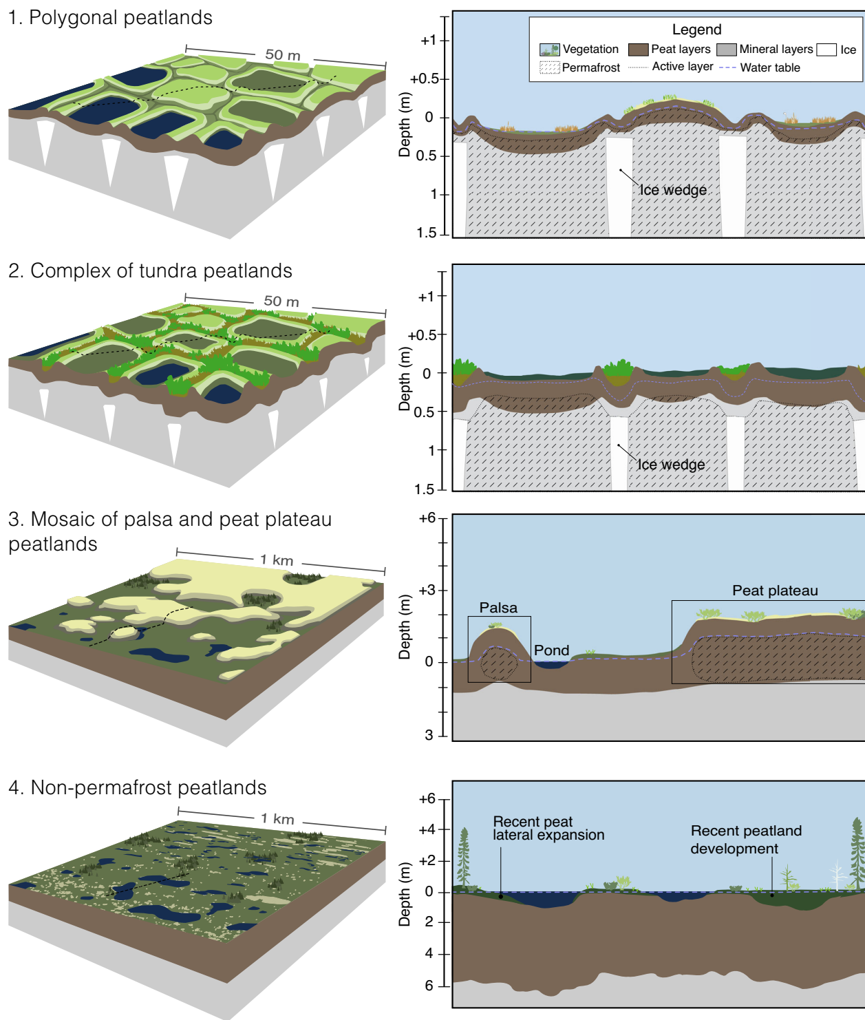
Fig. 4 | Peatland contrasting states found along the transect. Peatlands are terrestrial ecosystems in which waterlogged conditions prevent plant material from fully decomposing. Along the latitudinal transect, they range from polygonal peatlands shaped by the dynamics of ice-wedge networks to peatlands completely devoid
