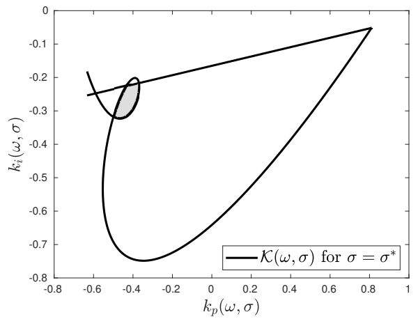
(b) \sigma -stable region for \sigma^* < \hat{\sigma} .
