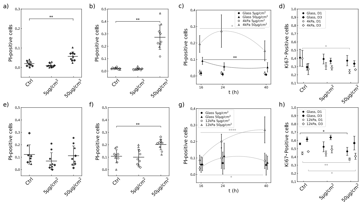
Fig. 7 NPs increase cell death and decrease the number of cycling cells in a more pronounced way when the cells are grown on a soft matrix. (a-d) U87-MG cells. (e-h) NIH 3T3 cells. (a,e) Ratio of dying cells (PI positive) when grown on glass, at D1 seeding density, 24 h post exposure to the NPs. Data from independent experiments are shown with different symbols. (b,f) Idem for cells grown on a soft substrate, of 4 kPa for the U87-MG cells and of 12 kPa for the NIH 3T3 cells. (c,g) Time evolution of the ratio of dying cells. (d,h) Proportion of cells engaged in the cycle (KI-67 positive) for two cell densities, D1 and D3. In (c,d,g,h), bars denote the standard deviation ( n=3 ) and significant differences are labeled in back for the glass conditions and in grey for the soft conditions. *, **, *** and **** denote significance with respectively p < 0.05 , 0.01 , 0.001 and 0.0001 . Only significant variations are labeled.
