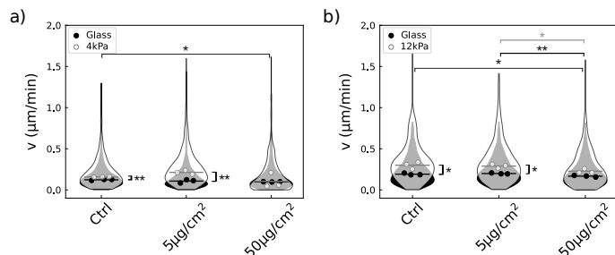
Fig. 8 Cell motility is slowed down when exposed to the highest concentration of NPs. (a) Distributions of instant velocities of the U87-MG cells captured 14 h post exposure to the NPs during 4 h with 1 h lapse, grown either on glass (dark background) or on 4 kPa substrate (white background). The dots show the medians of each of the independent experiments ( n=3 ). The horizontal bars show the mean of the medians. Only significant differences are labeled. Significant differences are labeled in back for the glass condition and in grey for the soft condition. (b) Same as in (a) for the NIH-3T3 cells. * and ** denote significance with respectively p < 0.05 and 0.01 .
