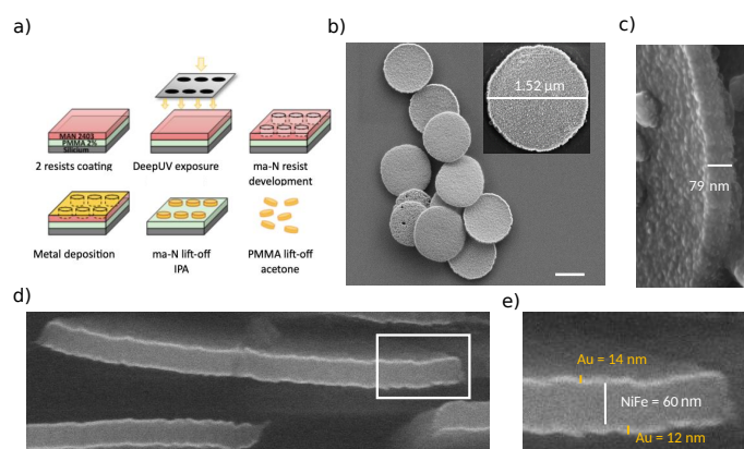
Fig. 1 (a) Nanofabrication process of the vortex microdiscs. (b–c) SEM images after particle release from the wafer showing top (b) and side (c) views of the NPs. Scale bar: 1 μm. (d) View of the lateral cross-section of particles, obtained with FIB-SEM. (e) Zoom of the region enclosed in the white rectangle in (d).
