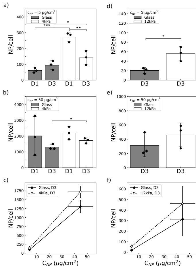
Fig. 6 Quantification of the number of NPs per cells in (a – c) U87-MG and (d – f) NIH 3T3 cell lines grown on a glass or a soft bottom at two seeding densities, D1 and D3. (a,d) Cells are exposed to 5 \mu\text{g}/\text{cm}^2 NPs. (b,e) Cells are exposed to 50 \mu\text{g}/\text{cm}^2 NPs. (d, e) The reduced interaction of NIH 3T3 cells with NPs did not allow to obtain a significant signal-to-noise ratio at D1. Only D3 data are therefore displayed. Symbols show independent experiments ( n=3 ). (c,f) NPs loading increases with NPs concentration whatever the substrate for the two cell lines. (c) U87-MG cells and (f) NIH 3T3 cells seeded at D3. Vertical errorbars show the standard deviation ( n=3 ). Horizontal error bars show the standard deviation in the concentration of mother solutions of NPs ( n=5 ). *, ** and *** denote significance with respectively p < 0.05 , 0.01 and 0.001. Only significant variations are labeled.
