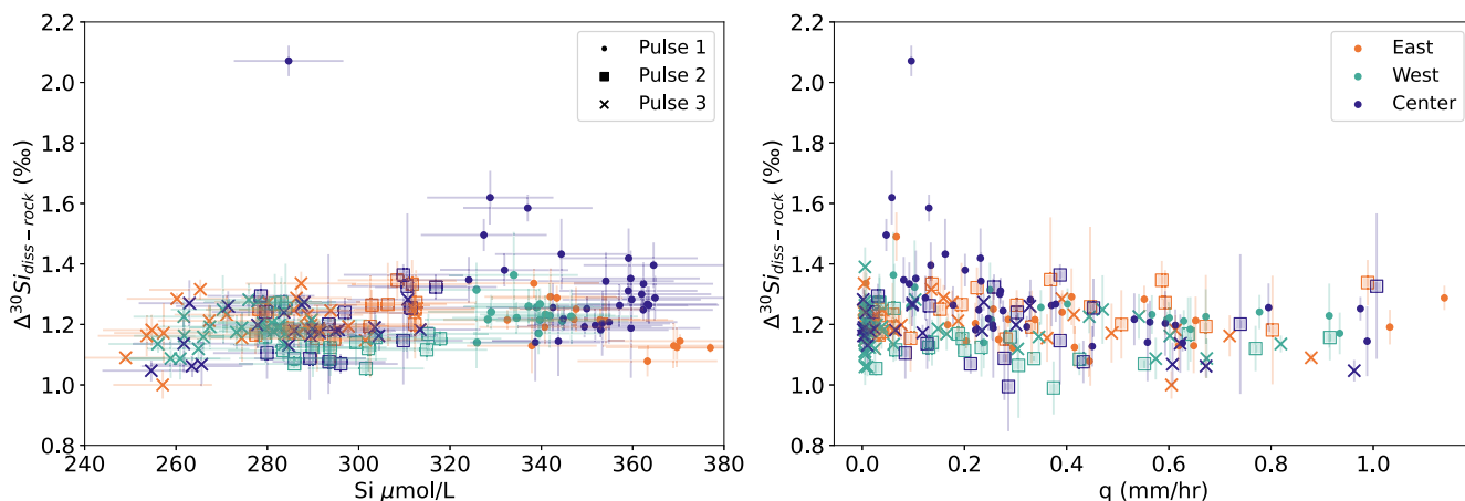
Fig. 3. Left \Delta^{30}\text{Si}_{\text{diss-rock}}(\text{‰}) against dissolved Si ( \mu\text{mol/L} ) Right: \Delta^{30}\text{Si}_{\text{diss-rock}}(\text{‰}) against Q (mm/hr) for all three pulses. ‘•’ = Pulse 1, ‘□’ = Pulse 2, ‘x’ = Pulse 3. Error shown on Si concentrations and isotope ratios are described in Section 2.3.
