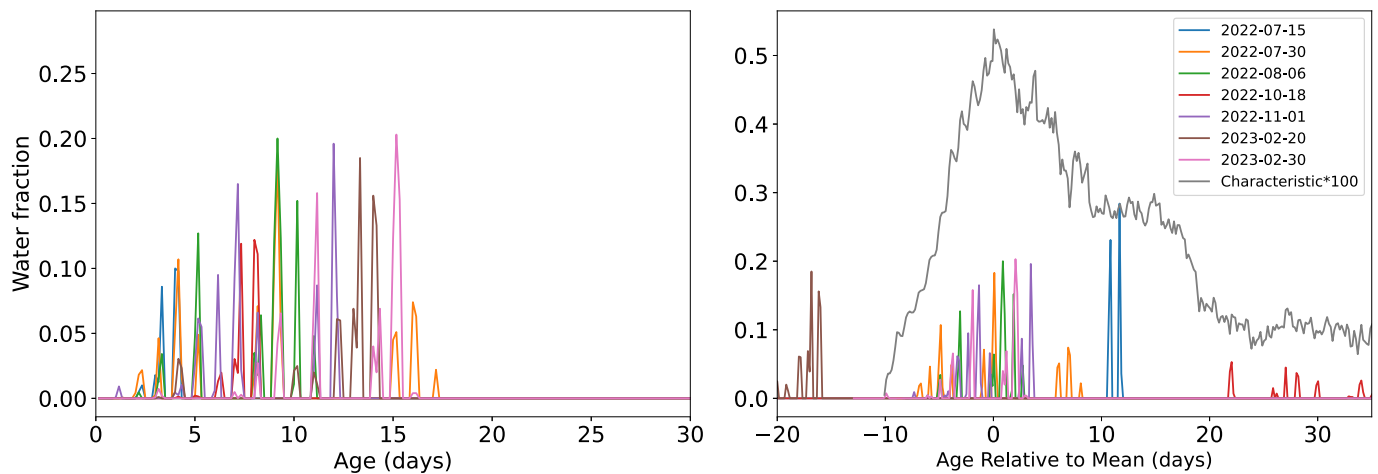
Fig. 7. Left: Modeled water transit time distributions at LEO for individual points in time. The Y-axis (water fraction) indicates the contribution of waters of a given age. Right: Same distributions plotted as age contributions relative to the mean age at the given time. Negative ages are contributions of water younger than the mean; positive ages are contributions of water older than the mean. Characteristic TTD scaled by 100 to show shape on same axis as individual TTDs.
