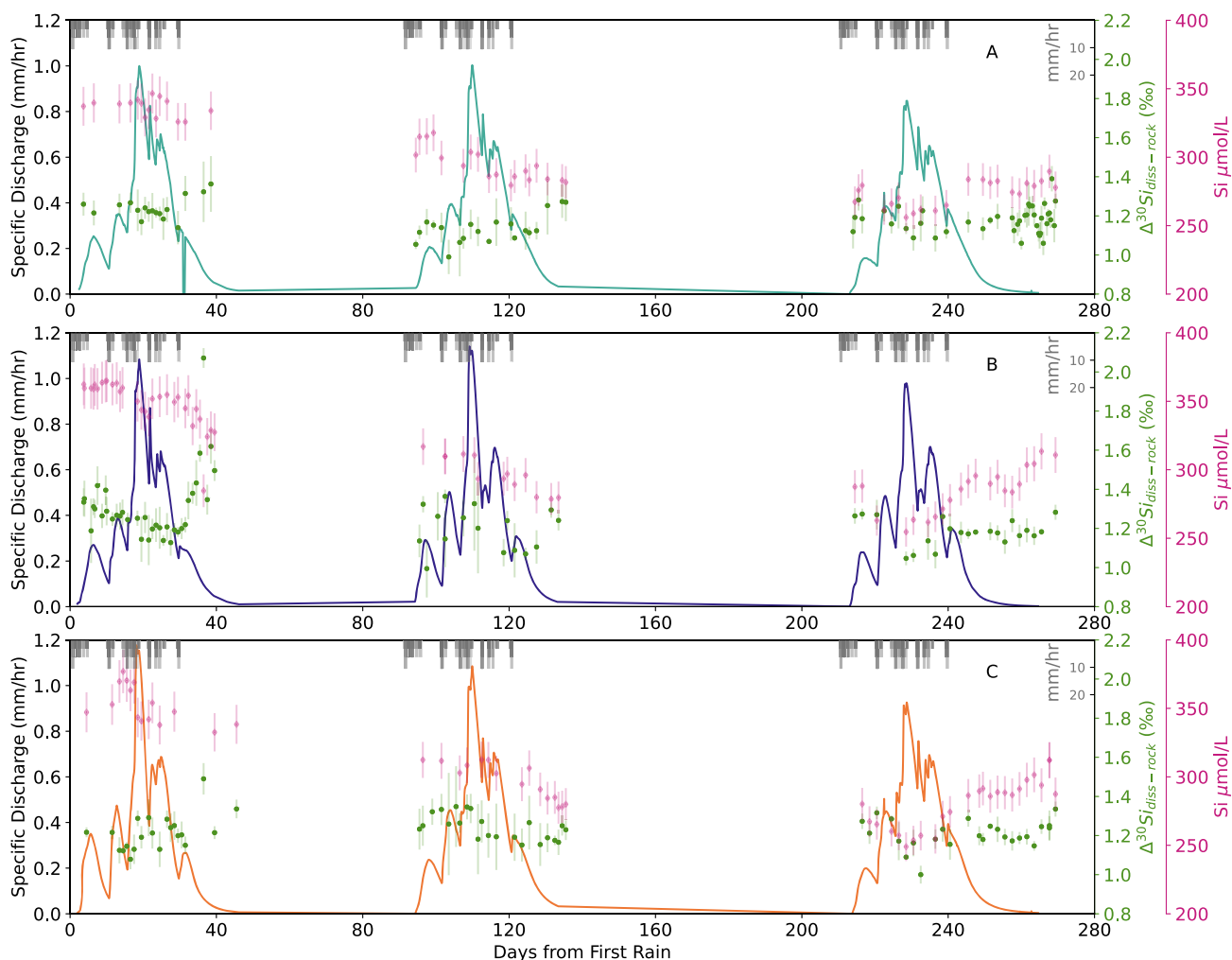
Fig. 2. (A) western, (B) central and (C) eastern hillslope timeseries of discharge (y1-axis), \Delta^{30}\text{Si}_{\text{diss-rock}} (y2-axis), and Si \mu\text{mol/L} (y3-axis). Green bars represent 95 % confidence interval. Error shown on Si concentrations and isotope ratios are described in Section 2.3.
