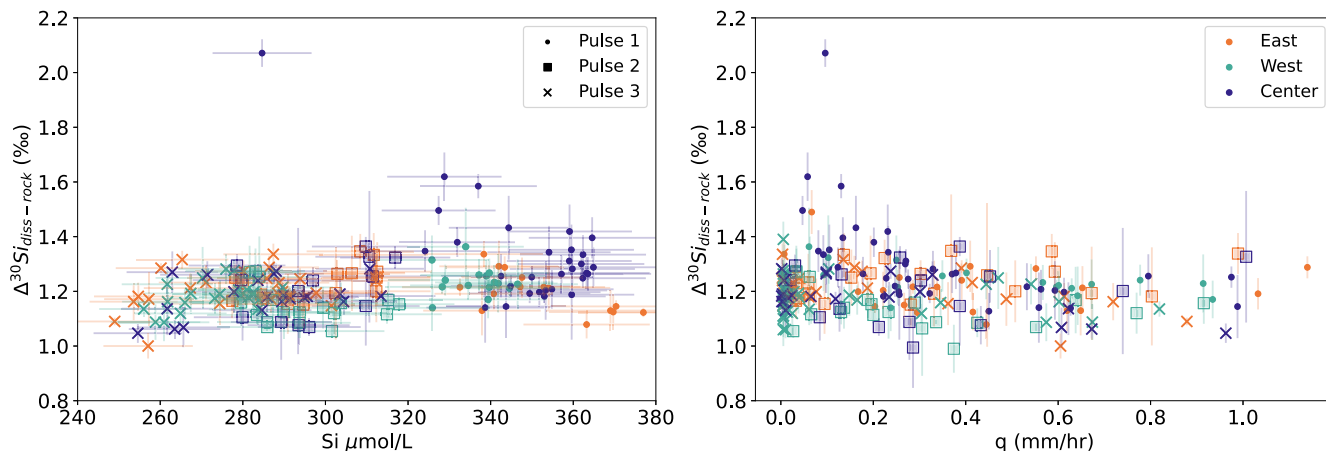
Fig. 3. Left \Delta^{30}\text{Si}_{\text{diss-rock}} (‰) against dissolved Si ( \mu\text{mol/L} ) Right: \Delta^{30}\text{Si}_{\text{diss-rock}} (‰) against Q (mm/hr) for all three pulses. ‘•’ = Pulse 1, ‘□’ = Pulse 2, ‘x’ = Pulse 3. Error shown on Si concentrations and isotope ratios are described in Section 2.3.
