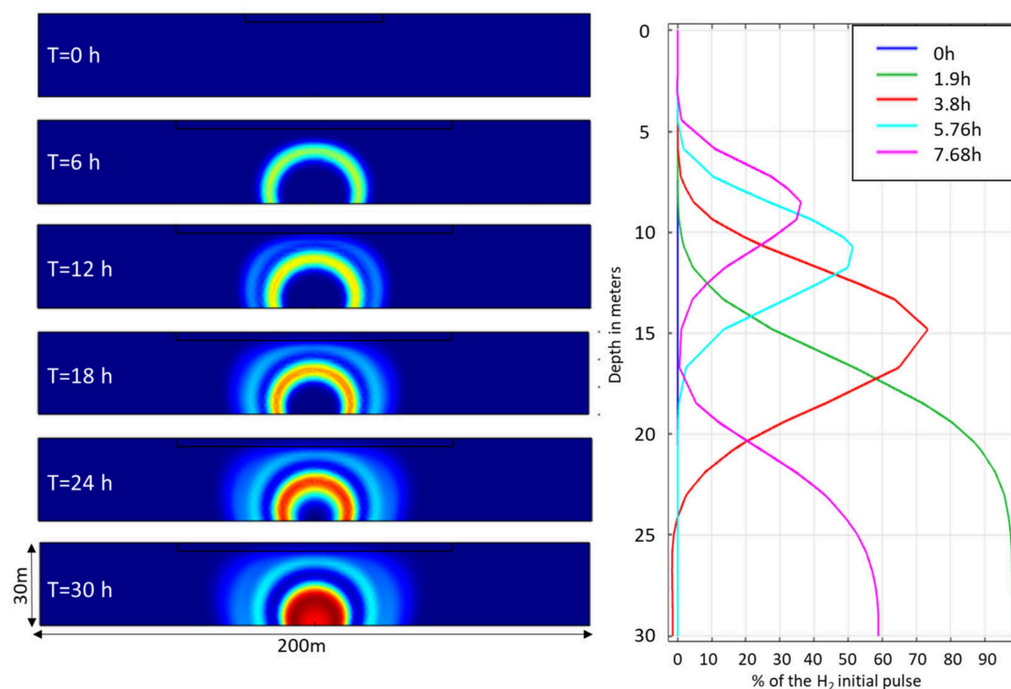
Figure 11. Signal with 4 pulse a day (6 h of gap); in that case, the distance between the two peaks is about 15 m. These figures come from the work performed in 2019 by A. Myagkiy but were not included as figures in the original paper [35]. In this model, a shaly bed in the central part of the model slows down the upward flow and precludes H 2 escape due to high microorganism consumption. It is not the case in the Colombian foreland. Left, the color code from red (100%) to blue (0%) indicates the ratio of the H 2 pulse that reach this point.
