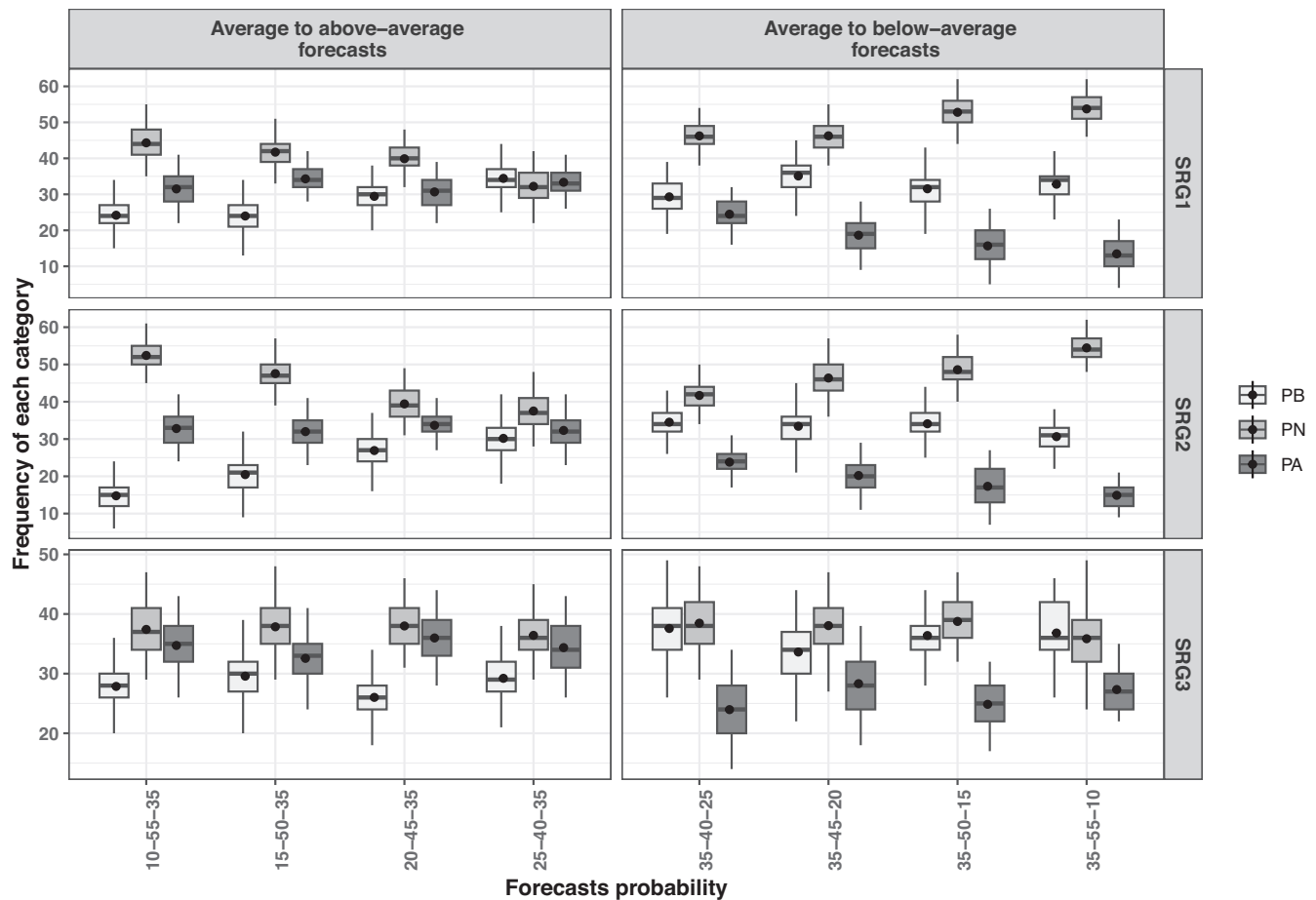
FIGURE 8 Frequencies (by conditionally generating 1000 simulations of 100 JAS daily rainy seasons for each forecast and both locations) of the below-average (PB), average (PN) and above-average (PA) categories, as functions of average West African RCOF seasonal rainfall forecast formats. The dots indicate the average frequencies for each category
