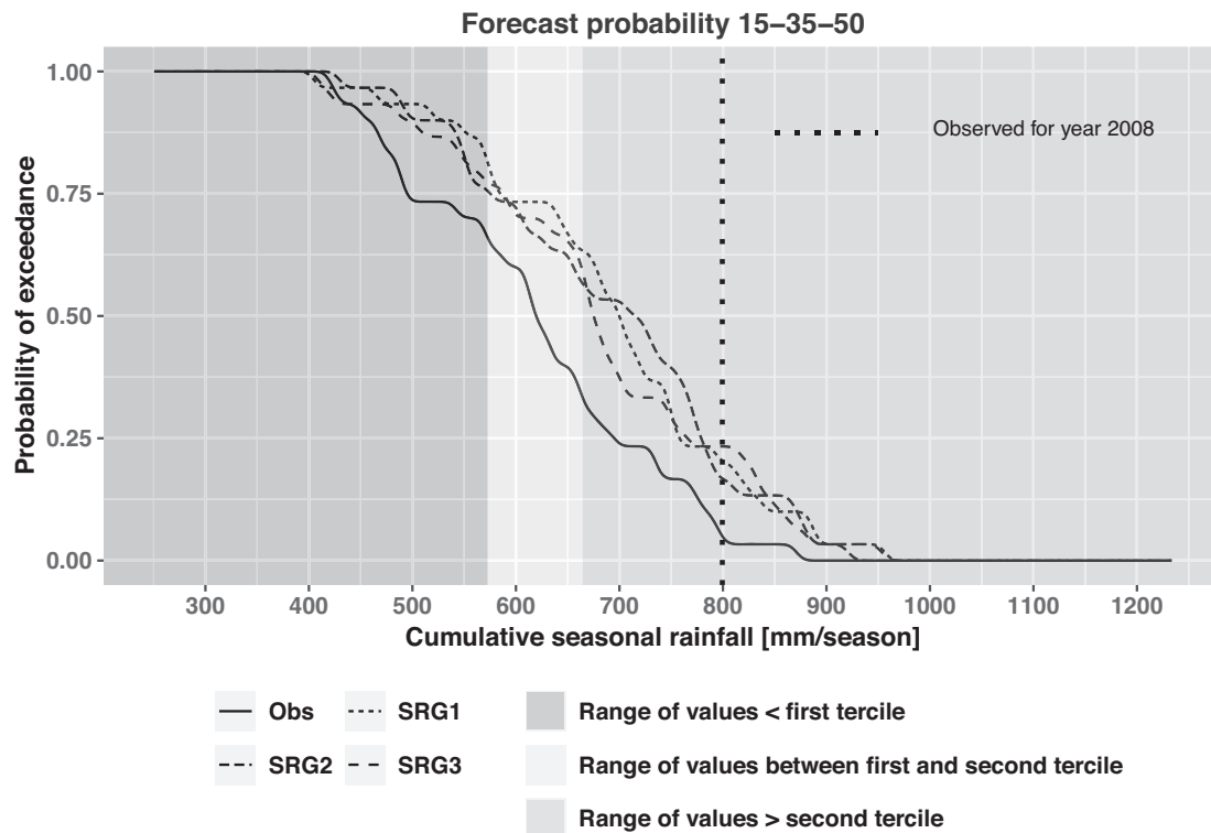
FIGURE 10 Comparison between the climatology CDF and the CDF for the seasonal amounts generated from the stochastic disaggregation models for rainfall (SRG) conditioned on the West African RCOF seasonal rainfall forecast probability (15–35–50 for the JAS season of the year 2008 at Kandi). Period 1971–2000 for climatology (Obs) and 30 disaggregated JAS seasons for SRGs. The cumulative seasonal rainfall for 2008 is shown in a dashed vertical line
