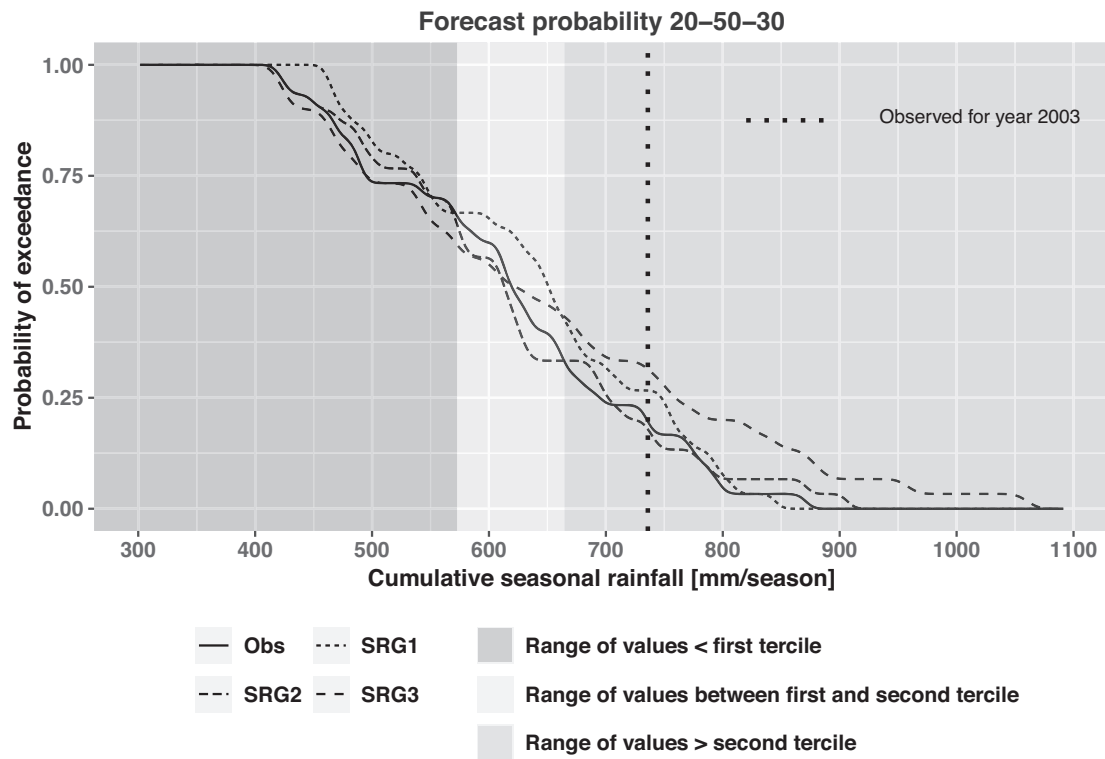
FIGURE 11 Comparison between the climatology CDF and the CDF for the seasonal amounts generated from the stochastic disaggregation models for rainfall (SRG) conditioned on the West African RCOF seasonal rainfall forecast probability (20–50–30 for the JAS season of the year 2003 at Kandi). Period 1971–2000 for climatology (Obs) and 30 disaggregated JAS seasons for SRGs. The cumulative seasonal rainfall for 2003 is shown in a dashed vertical line
