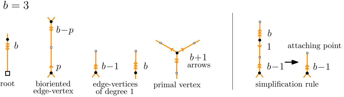
Figure 12: Environments of the various vertices in a b -arrow tree. For simplified b -arrow trees, non-root half-edges with b arrows are removed as shown on the right.
