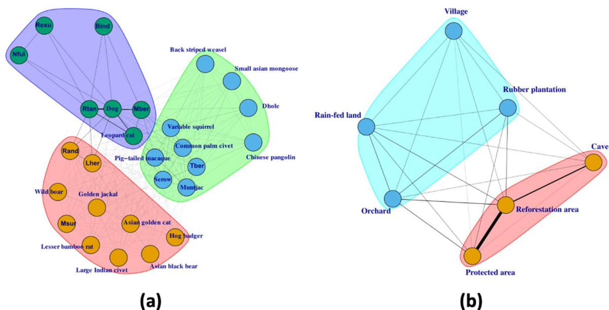
Figure 8. Unipartite networks of (a) mammal species and (b) habitats with modules differentiated by colours. The links between mammal species depict shared habitats, while the links between habitats depict shared mammal species (vertices were placed according to the Fruchterman–Reingold algorithm). Bind: Bandicota indica ; Lher: Leopoldamys herberti ; Mber: Menetes berdmorei ; Msur: Maxomys surifer ; Nful: Niviventer mekongis ; Rada: Rattus andamanensis ; Rexu: Rattus exulans ; Rtan: Rattus tanezumi ; and Tber: Tupaia belangeri .
