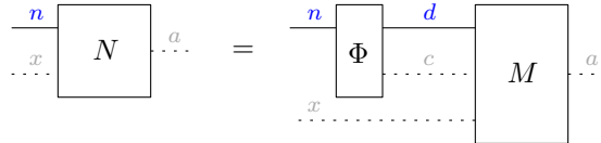
FIGURE 12. Compressibility of measurements. The quantum (solid) wires have dimensions indicated in blue.
