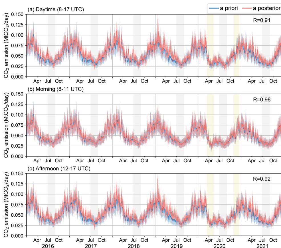
Figure 4. Daily estimates of fossil fuel CO 2 emissions over the greater Paris region when assimilating (a) daytime (08:00–17:00 UTC), (b) morning (08:00–11:00 UTC) and (c) afternoon (12:00–17:00 UTC) CO 2 concentration observations. The blue line and shading show the prior flux according to the Origins.earth inventory together with its assumed uncertainty. The pink and shading show the posterior estimates with their uncertainty ranges. The yellow shaded areas are the two COVID-19 lockdown periods in France. The grey shaded areas are the summer holidays in July and August.
