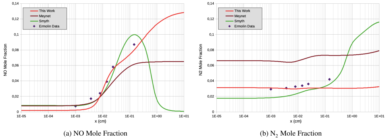
Figure 9: Profiles of NO and N 2 in the AP flame at 0.6 atm and initial temperature 533. Symbols: experiment [5]. Lines: model prediction.
