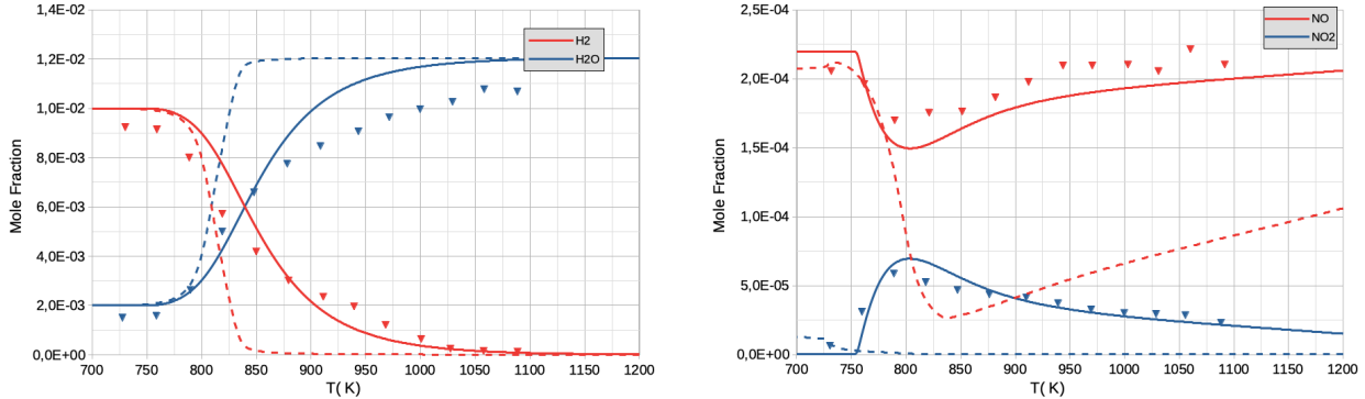
Figure 3: Reaction products of the mixture \text{H}_2 (1%) / \text{O}_2 (1%) / \text{N}_2 doped by 220 ppm of \text{NO} in a jet-stirred reactor at 10 atm, residence time 1s, variable temperature. Symbols: experiment [24]. Solid lines: present model. Dashed lines: Gross model
