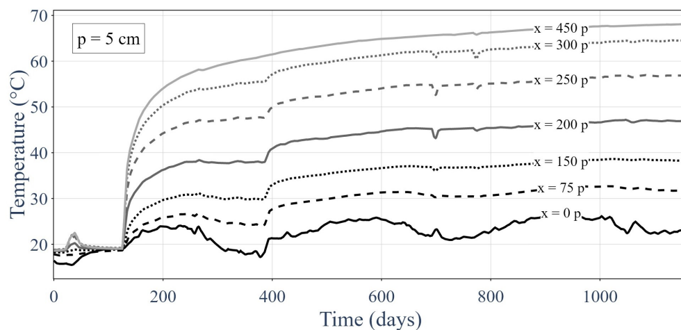
Figure 8. Thermal responses of the optic fiber sensor at set sample points over time.
