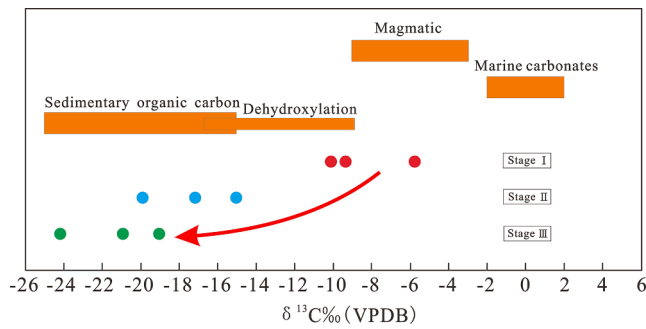
Fig. 13. Comparison of \delta^{13}\text{C} values of \text{CO}_2 in the fluid inclusions trapped in quartz from three hydrothermal stages in the Suixian Mo deposit with four primary carbon sources (modified after Veizer et al., 1980; Taylor, 1986; Ohmoto, 1972).
