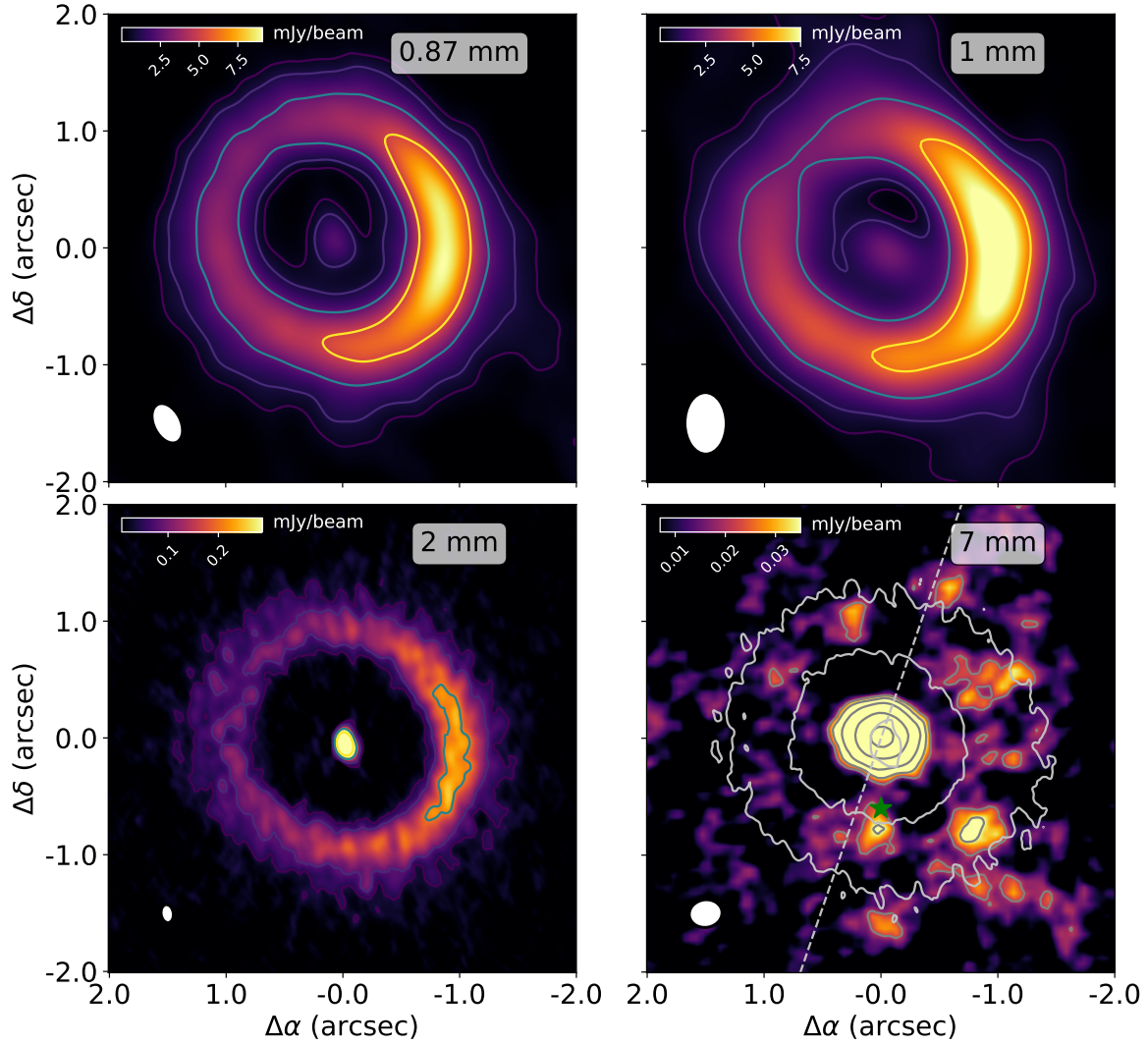
Fig. 1. Continuum maps at millimeter wavelengths. Top left: ALMA map at 0.87 mm. Top right: NOEMA map at 1.1 mm. Bottom left: ALMA map at 2.2 mm. Bottom right: VLA map at 7 mm. The light gray contours in the bottom right panel depict 5\sigma continuum emission at 2.2 mm from our ALMA map. The gray dashed line marks the position of the centimeter jet detected by Rodríguez et al. (2014). The green star marks the position of the tentative protoplanet proposed by Currie et al. (2022). The synthesized beam is shown in the bottom left corner of each map. Contour levels in the 0.87, 1.1, and 6.8 mm maps are 5, 10, 25, and 50\sigma . The 2.2 mm map only shows 5, 10, and 25\sigma levels. The map of the VLA emission at 7 mm also includes 3\sigma contour levels. In all maps, the color bar indicates flux in \text{mJy beam}^{-1} .
