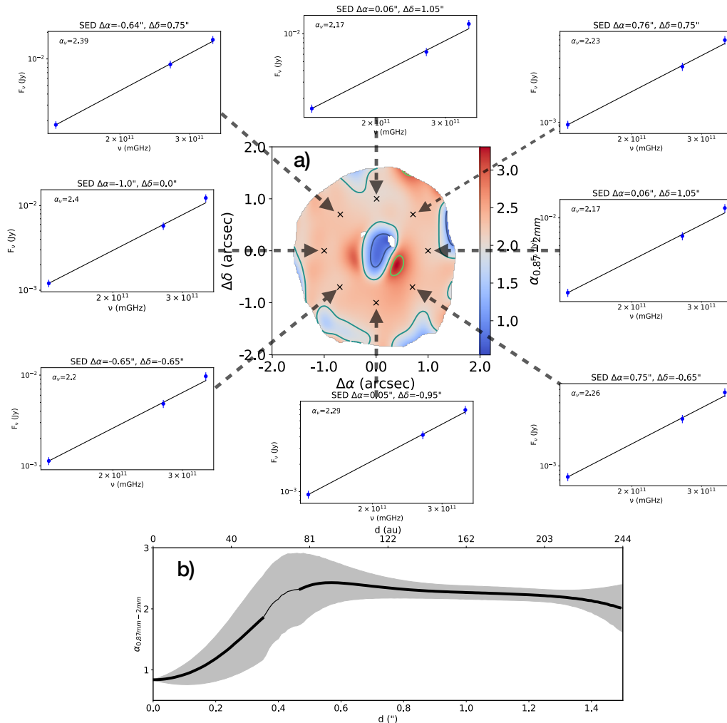
Fig. 7. Spectral index map computed using the 0.87, 1.1, and 2.2 mm data. (a) The resulting map with insets showing the SED at different positions in the disk. (b) Radial profile of the spectral index map computed using the 0.87, 1.1, and 2.2 mm data.
