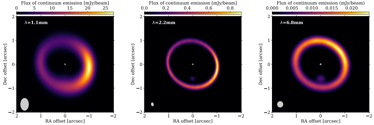
Fig. 9. Synthetic maps of dust continuum emission at 1.1 (left), 2.2 (center), and 6.8 mm (right) with the same beams as the NOEMA and ALMA images shown in Fig. 1, which are shown as gray ellipses in the lower left corner of each panel.
