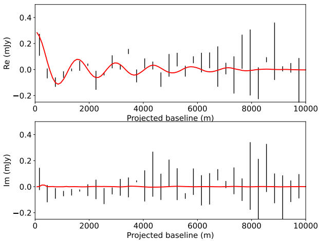
Fig. 10. Azimuthal average of the visibilities of our RADMC-3D model in the uv-plane. Top: Azimuthal average of the real part (red line, see Fig. 9) at 6.8 mm. We also show our observational data rebinned by a factor of three at 6.8 mm without the central source for comparison. Bottom: same as the top panel but for the imaginary part.
