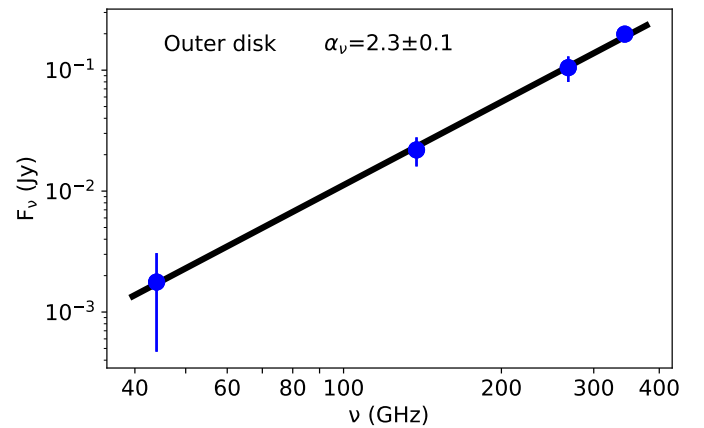
Fig. 5. Spectral energy distribution at millimeter wavelengths. Top: for the inner source. Bottom: for the outer disk. The blue dots represent our observations at different wavelengths, while the black line is a linear fit to the data.
