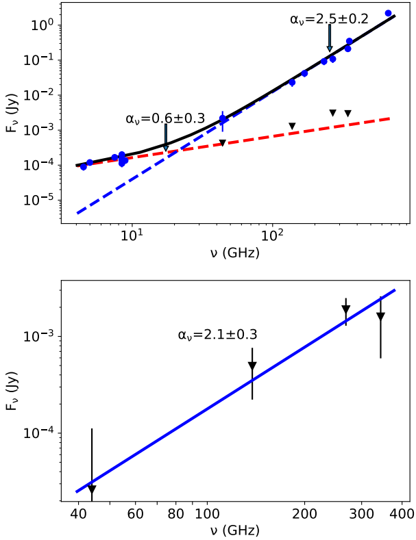
Fig. 11. Spectral energy distribution (SED) from the sub-millimeter to centimeter wavelengths. Top: SED of the whole disk. The thick red line depicts a fit to centimeter data, while the blue one shows a fit to sub-millimeter and millimeter data. The thick black curve shows the combined fit. Blue dots are observations from this paper (millimeter data) and the literature (sub-millimeter and centimeter). Black triangles are fluxes from the central source alone. Bottom: SED of the compact source towards the center after subtracting the free-free contribution.
