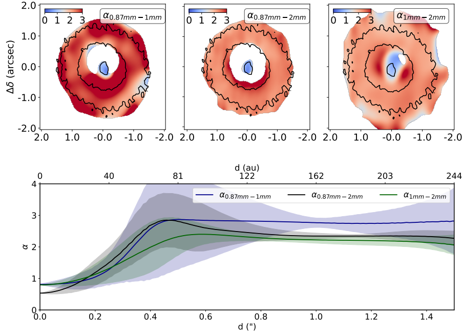
Fig. 6. Spectral index maps and profiles at millimeter wavelengths. Top: spectral index maps between 0.87 mm and 1.1 mm (left), 0.87 mm and 2 mm (middle), and 1.1 and 2.2 mm (right). Black contours depict 5\sigma continuum emission at 2.2 mm. Bottom: azimuthally averaged radial profiles of the spectral index maps between 0.87 and 1.1 mm, 0.87 and 2.2 mm, and 1.1 and 2.2 mm. The shaded areas represent the uncertainty in the radial profiles.
