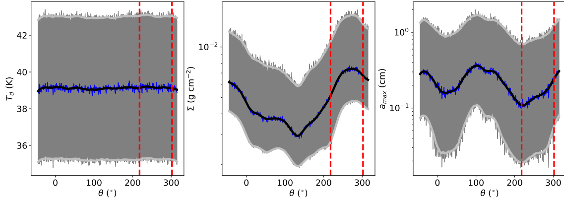
Fig. 8. Results from fitting the azimuthal profiles of continuum emission with 1D isothermal slab models. The blue curve depicts the best value at each azimuth and for each parameter, while the thick black curve represents a smoothed version after applying a Savitzky-Golay filter with a window length of 51 and a polynomial of order 3. The dark gray shaded regions represent the 16 and 84% confidence levels. The light gray curves represent a smoothed version of the confidence levels after applying the same Savitzky-Golay filter. The red vertical dashed lines show the approximate azimuthal extent of the dust trap as traced by the 0.87, 1.1, and 2.2 mm continuum maps.
