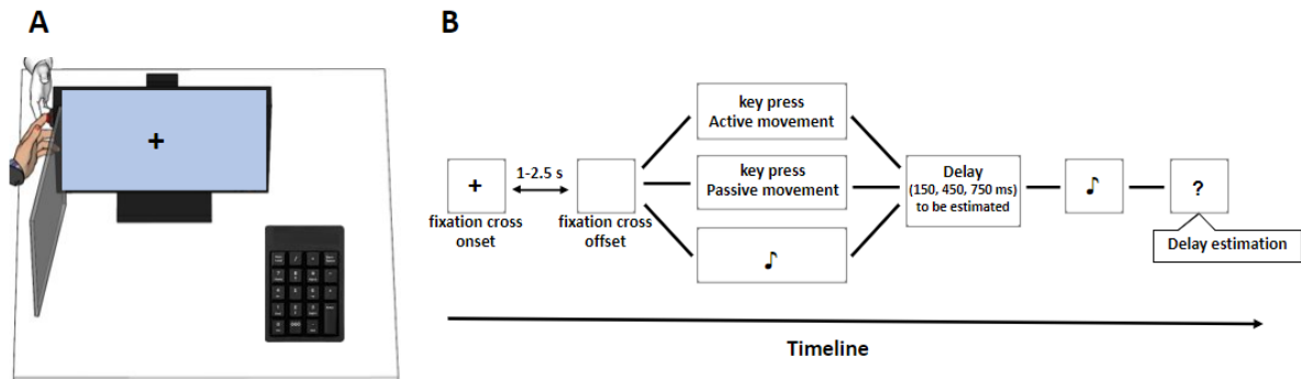
Figure 1. Set-up (A) and the three experimental conditions (B) of Experiment 1. (A) The set-up is shown here for the passive movement condition. (B) Schematic illustration of a trial in the three conditions: active movement, passive movement and external sensory event conditions. Note that the same number of events occurred during a trial for all the conditions.
