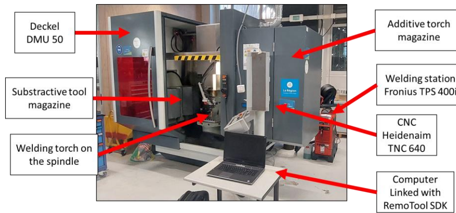
Figure 2 : Machine hybride
