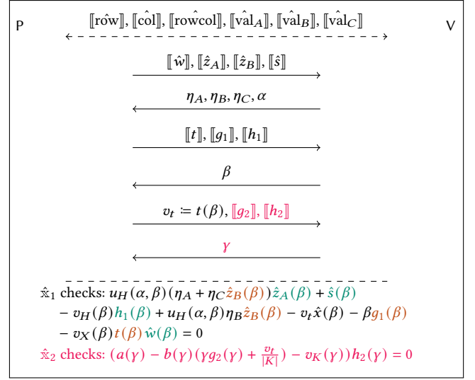
Figure 4: The \hat{\mathcal{R}}_{\text{lin}} -PIOP Marlin, where: v_H (resp. v_K, v_X ) denotes the vanishing polynomial of the subgroup H (resp. K, X ) of \mathbb{F} ; u_H is the formal derivative of v_H ; the polynomials a and b are computed using the index polynomials and the coins \alpha and \beta . We highlight the delegation phase , the core and right polynomials of \hat{\mathbb{x}}_1 .
