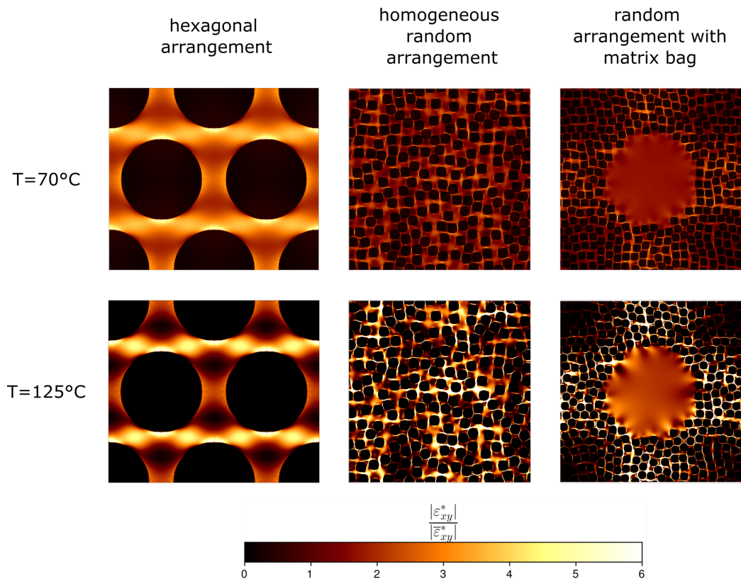
Figure 11: Normalized strain field \frac{\varepsilon_{xy}}{\bar{\varepsilon}_{xy}} extracted from FFT calculations for hexagonal (left), random (middle) and random with circular matrix bags (right) microstructures. The considered temperatures are 70°C (top) and 125°C (bottom) and the fiber volume fraction is 53% in all cases.
