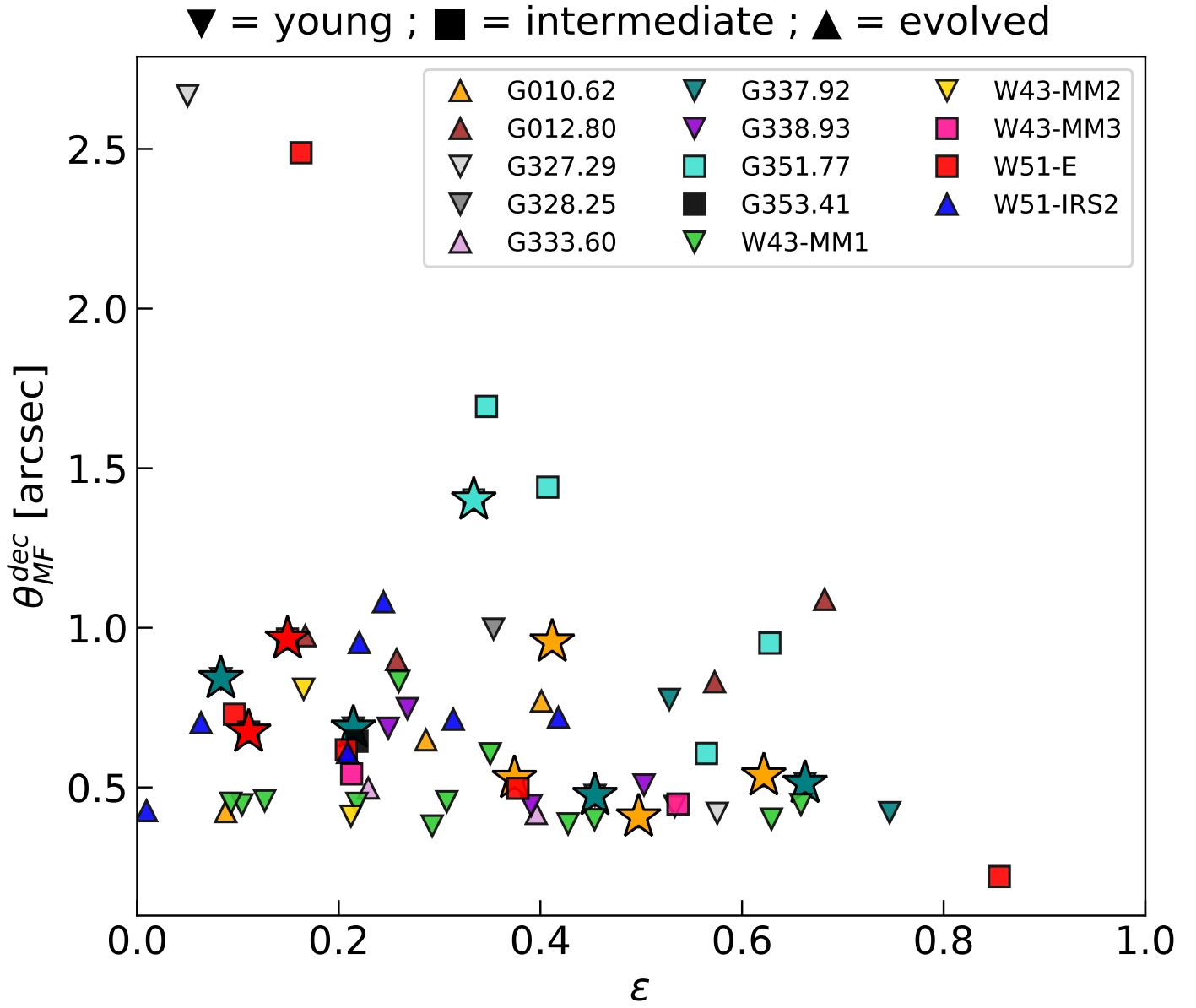
Fig. E.1: Methyl formate deconvolved source sizes ( \theta_{MF}^{dec} ) as a function of their ellipticity ( \epsilon ). The different symbols represent the different evolutionary stages of the protoclusters: young, intermediate, or evolved, as shown on top of the figure. The methyl formate sources that are not associated with compact continuum cores are shown with stars. The sources for which \theta_{MF}^{dec} is lower than half of the line cube beam size are not shown in the figure.
