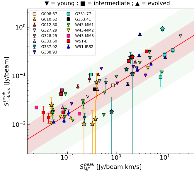
Fig. 14. Peak continuum flux density at 1.3 mm vs. peak flux extracted in the moment 0 maps of \text{CH}_3\text{OCHO} by GExt2D. The different symbols represent the different evolutionary stages of the protoclusters: young, intermediate and evolved, as indicated on top of the figure, while the stars shows the methyl formate sources that are not associated with any compact dust continuum core. The red line shows a weighted linear fit, while the red and green shaded regions show a factor of 2 and 5 deviation from this fit, respectively.
