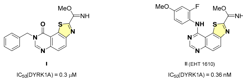
Figure 3. Structures of methyl 8-benzyl-9-oxo-8,9-dihydrothiazolo[5,4- f ]quinazoline-2-carbimidate ( I ) and methyl 9-[(2-fluoro-4-methoxyphenyl)amino]thiazolo[5,4- f ]quinazoline-2-carbimidate ( II ) used as references in this study.
