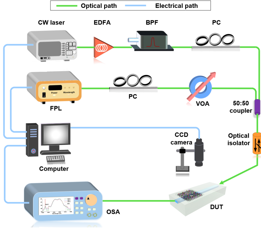
Figure 3. Experimental setup for OPA experiments. CW laser: continuous-wave laser. FPL: fiber pulsed laser. BPF: band-pass filter. PC: polarization controller. EDFA: erbium doped fiber amplifier. VOA: variable optical attenuator. DUT: device under test. CCD: charged-coupled device. OSA: optical spectrum analyzer.
