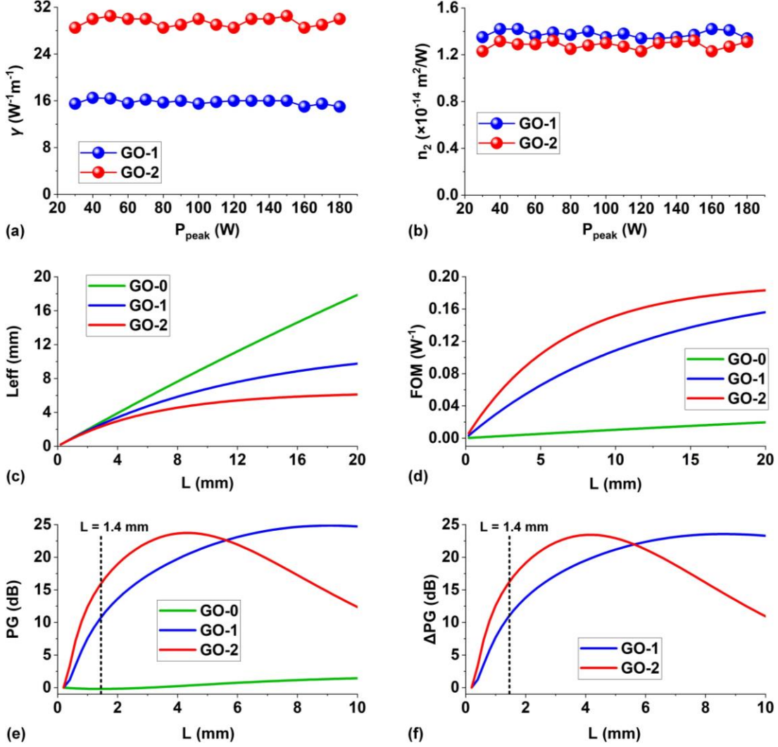
Figure 6. (a) Experimentally fitted nonlinear parameter \gamma of hybrid waveguides with 1 (GO-1) and 2 (GO-2) layers of GO as a function of pump peak power P_{peak} . (b) Kerr coefficient n_2 of films with 1 (GO-1) and 2 (GO-2) layers of GO versus P_{peak} . (c) Effective interaction length L_{eff} and (d) figure of merit FOM versus waveguide length L for the uncoated (GO-0) and hybrid waveguides with 1 (GO-1) and 2 (GO-2) layers of GO. (e) Parametric gain PG and (f) parametric gain improvement \Delta PG versus waveguide length L for the uncoated \text{Si}_3\text{N}_4 waveguide (GO-0) and the hybrid waveguides uniformly coated with 1 (GO-1) and 2 (GO-2) layers of GO. In (e) and (f), the pump peak power, CW signal power, and the wavelength detuning are P_{peak} = \sim 180 W, P_{signal} = \sim 6 mW, and \Delta\lambda = \sim -22 nm, respectively.
