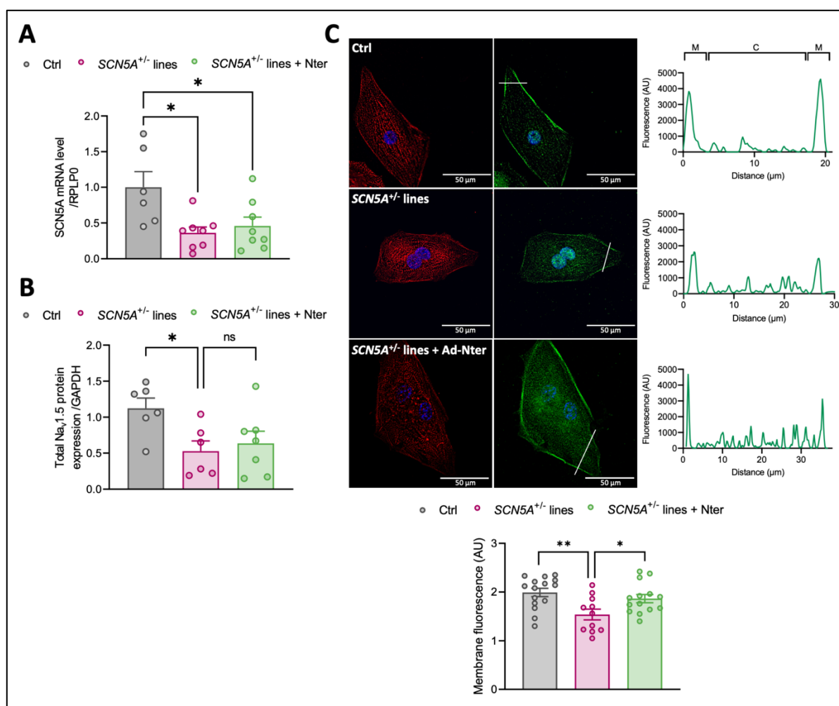
Figure 4. Na v 1.5 membrane expression was increased by Nter overexpression in SCN5A +/- iPSC-CMs A. SCN5A mRNA expression level in control (Ctrl) and SCN5A +/- iPSC-CMs transduced with Ad-GFP or Ad-Nter. Cts were normalized to hRPLP0 and the ratio vs. Ctrl ( 2^{-\Delta\Delta Ct} ) was then calculated; * P <0.05 ( One-way Anova test ) B. Western-blot analysis of Na v 1.5 expression normalized to GAPDH expression in Ctrl and SCN5A +/- iPSC-CMs transduced with Ad-GFP or Ad-Nter; ** P <0.01 ( One-way Anova test ). C, Left. Representative confocal images for immunostainings of \alpha -actinin (red) and Na v 1.5 (green) in Ctrl and SCN5A +/- iPSC-CMs transduced with Ad-GFP or Ad-Nter; Right. Fluorescence measurement of Na v 1.5 staining using ImageJ software; Bottom. Quantification of Na v 1.5 expression at the plasma membrane in Ctrl and SCN5A +/- iPSC-CMs transduced with Ad-GFP or Ad-Nter; * P <0.05, ** P <0.01 ( One-way Anova test ). All values were expressed as mean \pm SEM. N = 3 independent biological experiments per condition. The control iPSC-CMs are shown in gray, the SCN5A +/- iPSC-CMs + Ad-GFP in pink and the SCN5A +/- iPSC-CMs + Ad-Nter in green.
