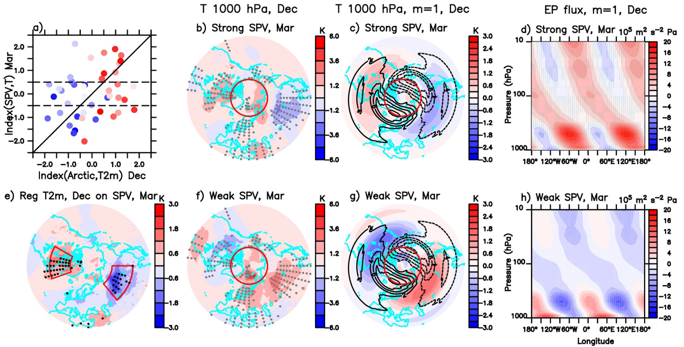
Figure 4. (a) Scatterplot of two normalized indices: the December 2 m temperature anomaly averaged between 70°N and 90°N (denoted as Index (Arctic, T2m)) and zero minus the March temperature anomaly averaged between 10 hPa and 50 hPa and between 70°N and 90°N (denoted as Index (SPV, T)). Blue (red) dots correspond to the 1979–2000 (2001–2022) period with the darker blue (red) dots corresponding to the oldest (newest) years of that period. Anomaly composites for (b), (c), (d) strong polar vortex (Index (SPV, T) in March greater than 0.5 standard deviations) and (f), (g), (h) weak polar vortex (Index (SPV, T) in March smaller than –0.5 standard deviations) during the recent period 2001–2022: (b), (f) anomalous 1,000 hPa temperature, gray dots representing regions where panels (b) and (f) are significantly distinct at the 99% confidence level following a two-sample two-tailed t -test, (c), (g) anomalous wave-1, 1,000 hPa temperature (shadings) and climatological wave-1 1,000 hPa temperature (black contours; interval: 2 K), (d), (h) anomalous vertical component of Eliassen–Palm flux F_p , averaged between 50°N and 70°N. The strong polar vortex composite in March is based on the following years: 2004, 2006, 2009, 2011, 2013, 2015, 2019, 2020, 2021 while the weak polar vortex composite in March contains the following years: 2005, 2008, 2014, 2016, 2018, 2022. (e) Regression of December 2 m temperature on Index (SPV, T) in March. The red boxes over Canada and Eurasia are used to compute indexes whose correlations with Index (SPV, T) are shown in Table 1. Data: ERA5 at monthly time scales.
