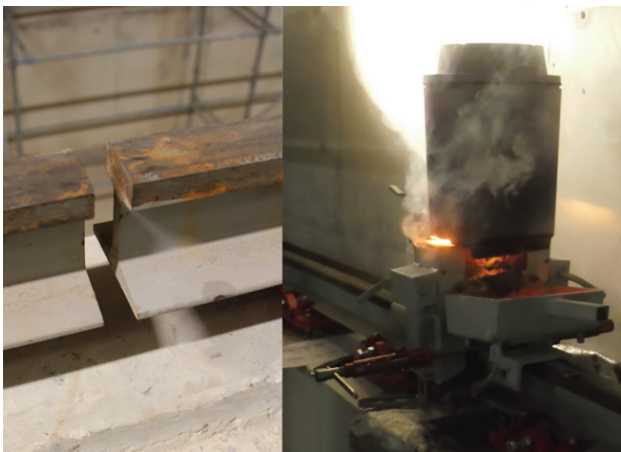
Figure 4. Rail welding
