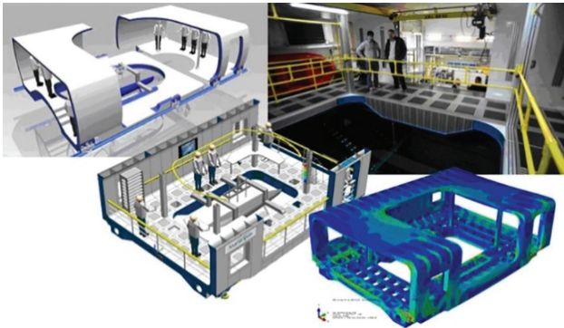
Figure 7. Development of the carriage design
