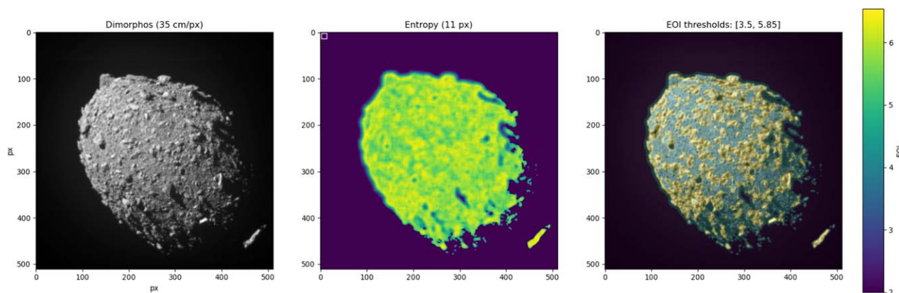
Figure 9. EOI measured on Dimorphos at 35 \text{ cm pixel}^{-1} . The thresholds in EOI values have been chosen to clearly separate boulders from pebbles.
