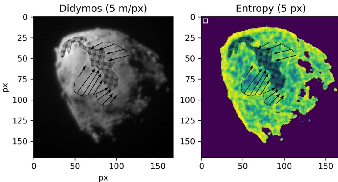
Figure 8. Example of a morphological unit identified on Didymos, overlaid on the original image and the map of EOI. The dotted area shows the contiguous smooth equatorial region. Dotted lines and arrows indicate putative mass wasting. A complete description of the geological units is available in O. S. Barnouin et al. (2023).
