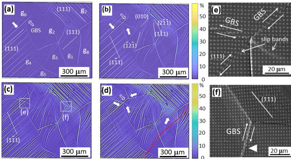
528 Figure 9: SEM and DIC characterization of deformation mechanisms at 200°C. (a), (b), (c) and (d) show the 529 cumulative evolution of localization patterns at respective axial strains of ca. 0.3 % (briefly after yielding), 1.5, 3, 530 and 5, respectively. Straight slip bands correspond to octahedral slip. Wavy cross slip bands represent cross-slip 531 involving octahedral and non-octahedral slip. Crystal slip transmitted across four neighboring grains is underlined 532 by one red dotted trajectory. Hollow arrows point to GBS localization. Plain arrows indicate crystal slip bands 533 aligned with grain boundaries subjected to GBS. The square-areas defined in (c) correspond to the SEM 534 micrographs in (e) and (f), where the interactions between GBS and crystal slip at triple junctions is evidenced. In 535 (e) the right hand GBS triggers on the left hand one octahedral (111) slip band. The left hand GBS triggers an 536 undetermined crystal slip band on the right hand. 537 538
