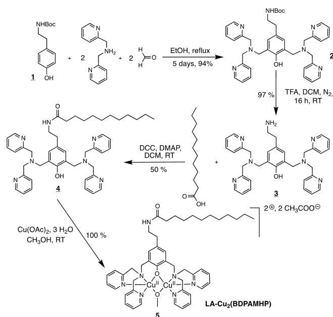
Scheme 1. Synthesis of di-copper(II)-N-(3,5-bis((2,2'-dipicolylaminomethyl)-4-hydroxy-phenethyl)lauramide LA- \text{Cu}_2(\text{BDPAMHP}) 5 .
