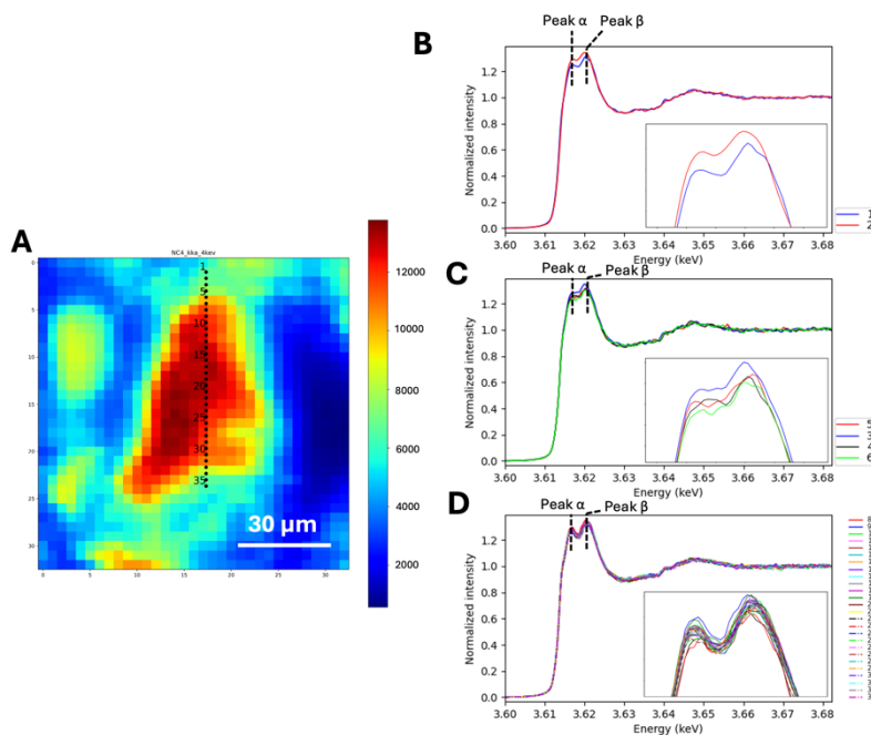
Figure 8: Comparison of XANES spectra at the K K-edge from the CW4 sample. A: K XRF elemental map with the position of the measured spectra. B: XANES spectra far from the edge of the grain. C: XANES spectra near the edge of the grain. D: XANES spectra measured inside the grain
