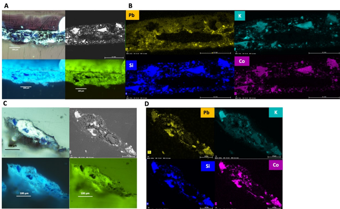
Figure 2: Observation of optical and electron microscopy of stratigraphic cross-sections of two samples prepared with siccative linseed oil, unaged (SLO) and aged for 23 days (SL4) and elemental analysis. A: Micrograph of sample SLO under white light, near UV light and UV light and SEM image of the cross-section. B: Individual elemental maps of the cross-section of the SLO sample. C: Micrograph of sample SL4 under white light, near UV light and UV light and SEM image of the cross-section. D: Individual elemental maps of the cross-section of the SL4 sample.
