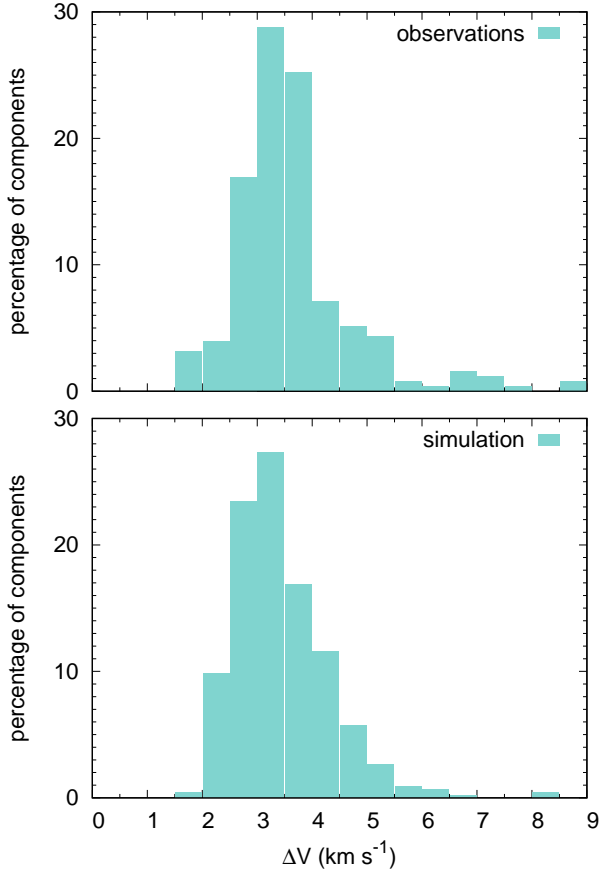
Fig. 7. Probability distributions of the full width at half maximum \Delta V of the 4232 Å line of CH + derived from the observations ( top panel ) and from synthetic spectra (see Fig. 6) computed across the standard simulation ( bottom panel ). The observational sample includes 254 velocity components extracted along 120 lines of sight by Federman (1982; Table 2), Lambert & Danks (1986; Table 1), Crane et al. (1995; Table 2), Pan et al. (2004; Table 4), Ritchey et al. (2006; Table 4), and Sheffer et al. (2008; Table 3). This dataset includes all the lines of sight where CH + has been observed (see Table A.1), except those observed or compiled by Gredel et al. (2002) and Rachford et al. (2002), who do not provide measurements of the CH + linewidth.
