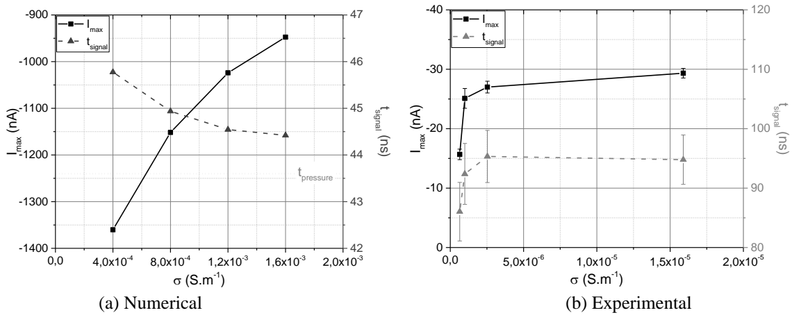
Fig. 14. Evolution of the maximum amplitude and the duration of the calculated signal according to water conductivity ( P_{\max}=1 \text{ MPa} ; t_{\text{pressure}}=43.56 \text{ ns} ) (a) and the values experimentally obtained according to glycerol conductivity (b).
